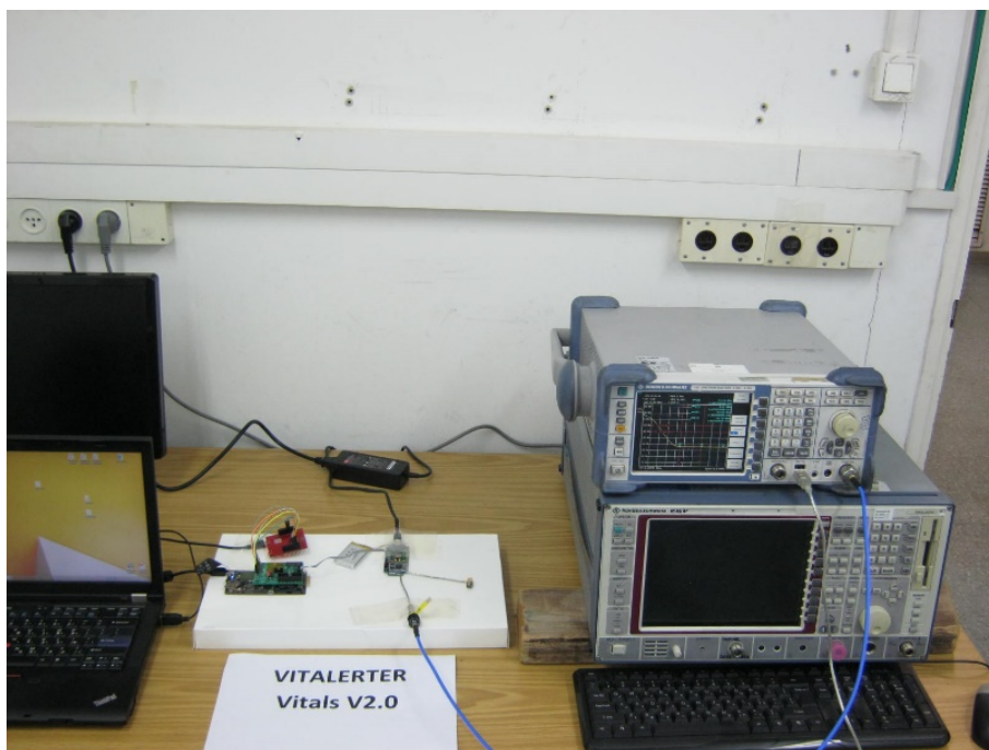
Conducted Emission From Antenna Ports Test
