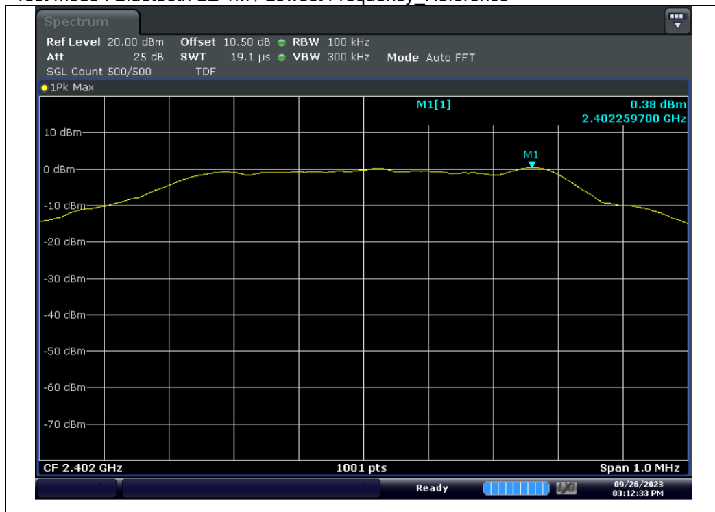
Test mode : Bluetooth LE 1M / Lowest Frequency _Reference
