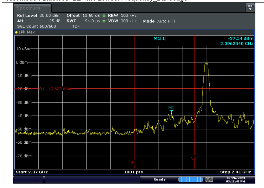
Test mode : Bluetooth LE 1M / Lowest Frequency _Bandedge
