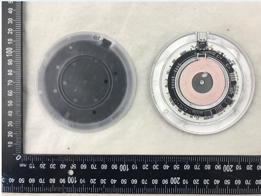
EUT UNCOVER VIEW 1 (Wireless charger)
