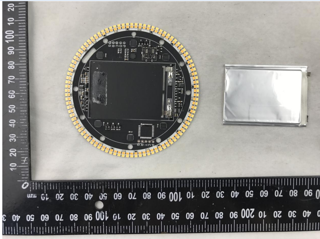
EUT UNCOVER VIEW 2 (Mirror)
