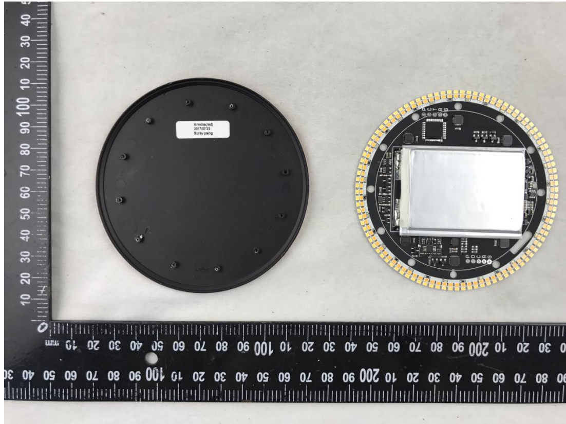
EUT UNCOVER VIEW 1 (Mirror)
