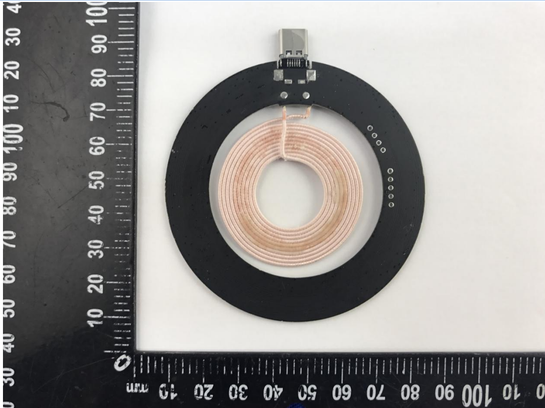
MAIN BOARD BACK VIEW (Wireless charger)
