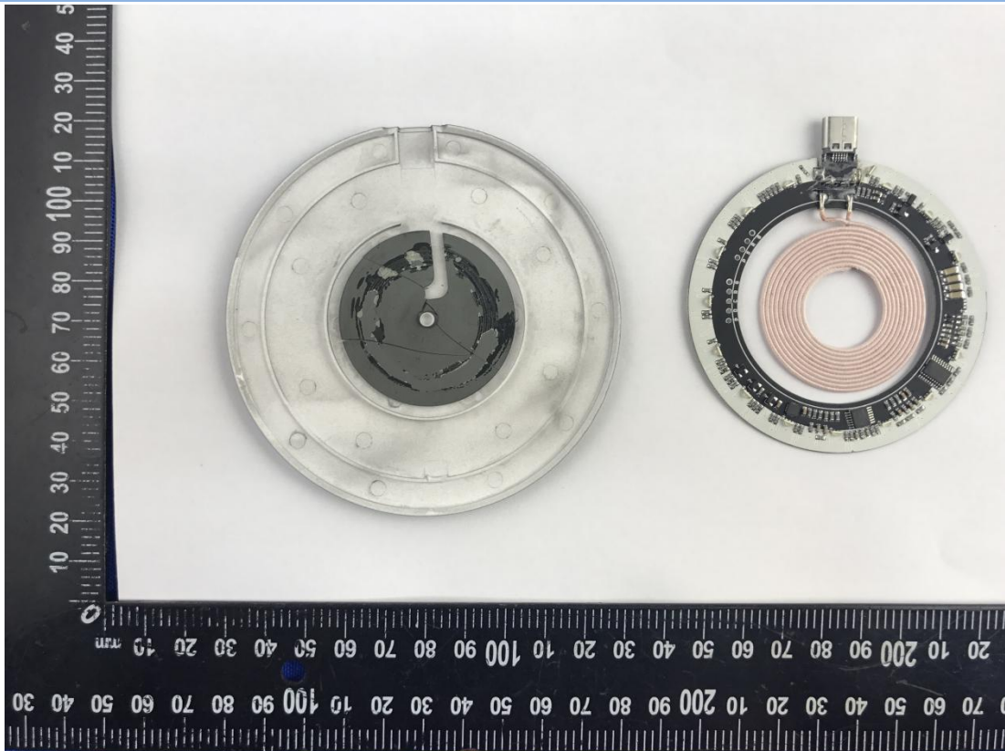
EUT UNCOVER VIEW 2 (Wireless charger)
