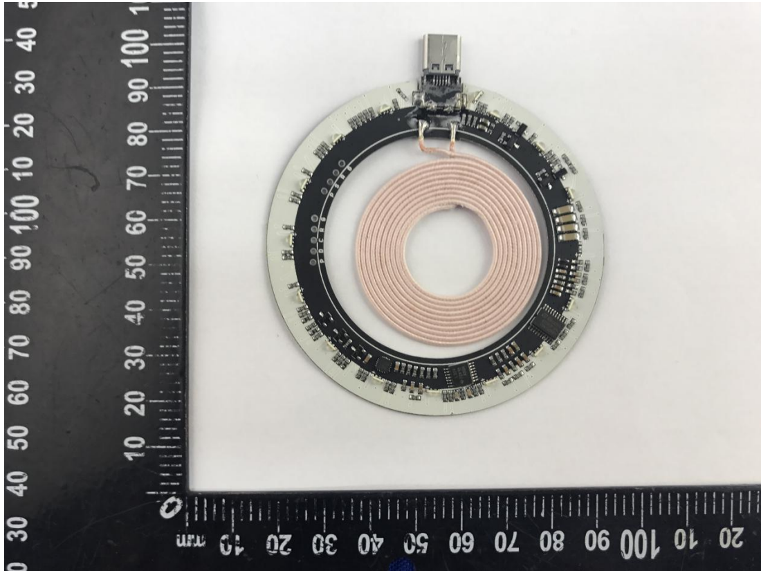
MAIN BOARD TOP VIEW (Wireless charger)
