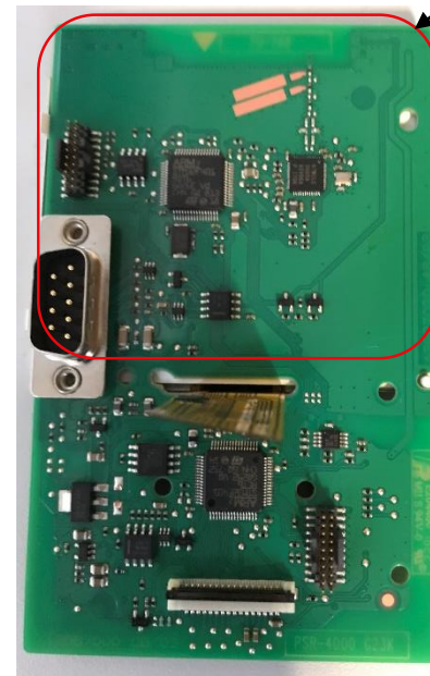
ICP with WiFi/BT + display - Back
