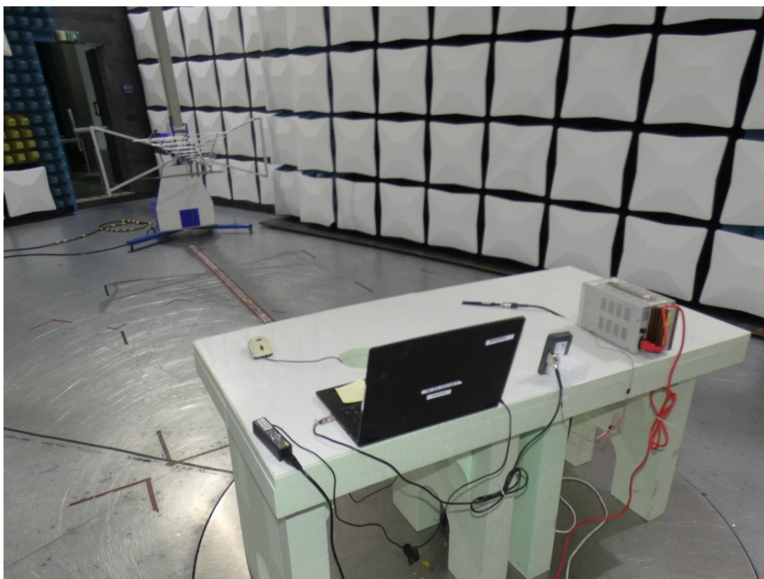
Photo 3: Test setup for radiated measurements below 1 GHz FCC 15b
