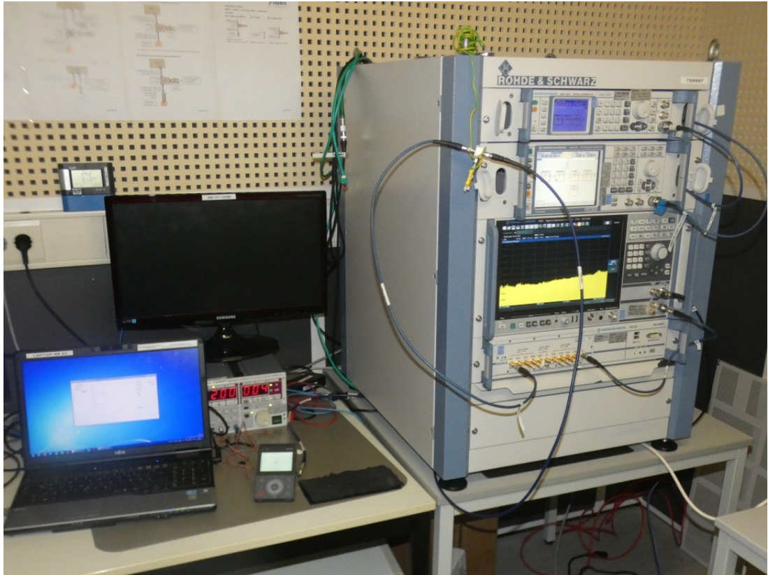
Photo 7: Test setup for conducted measurements
