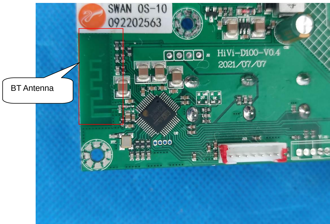
ANTENNA CLOSE-UP PHOTO-1
