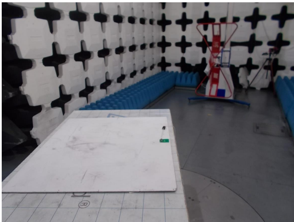
radiated emission test set-up (range 30MHz-1GHz)
