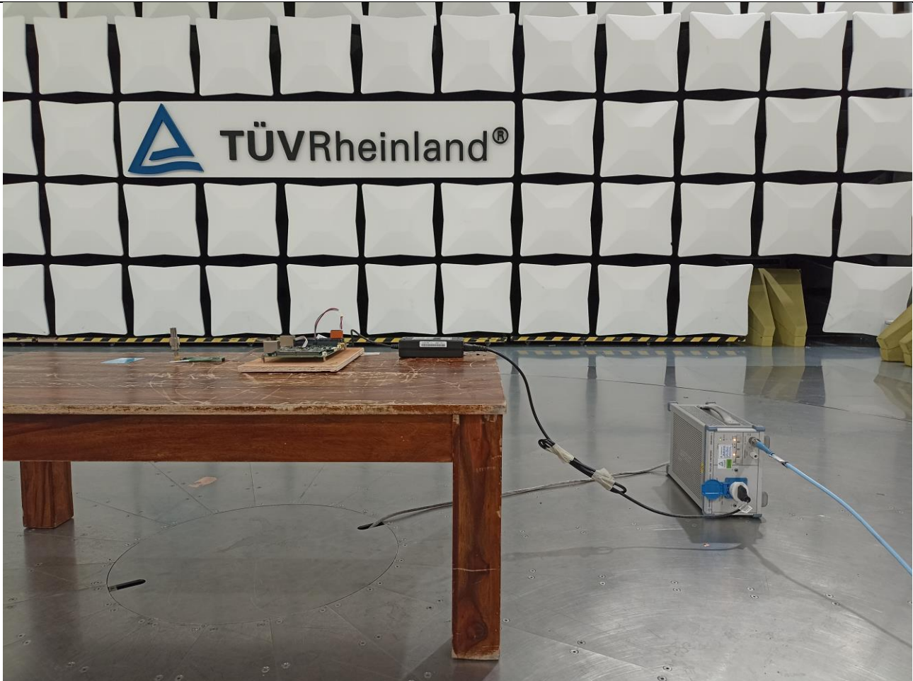
Emi cond test set-up photo
