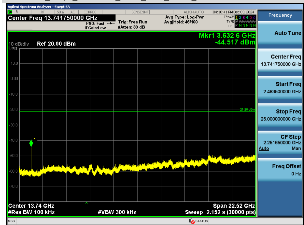
Test_Graph_802.11n40_ANT1_2422_MCS0_Higher Band Emissions
