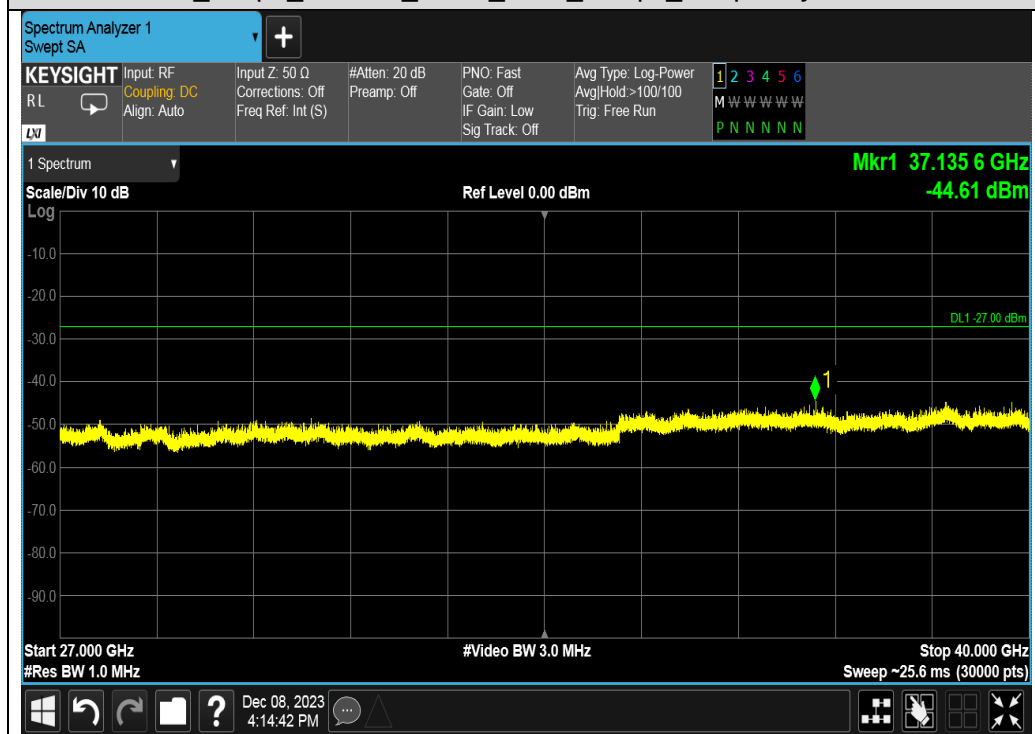
Test_Graph_802.11a_ANT1_5320_6Mbps_Frequency Band 5
