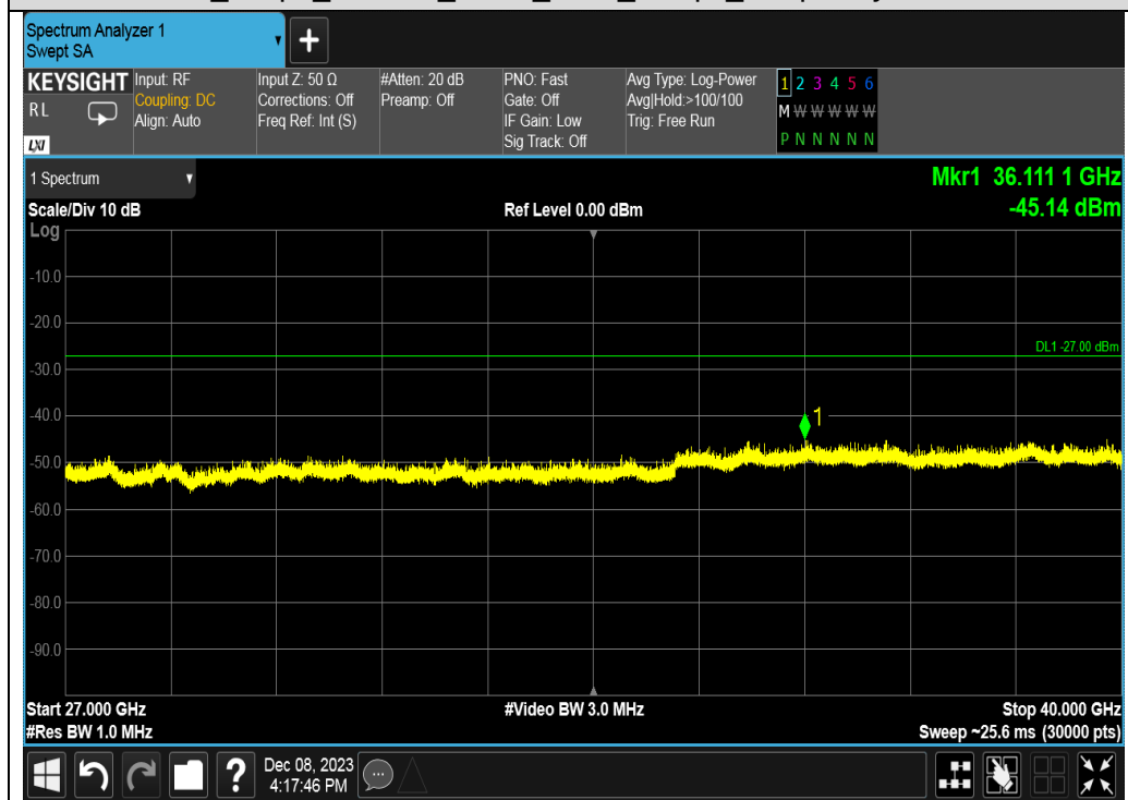
Test_Graph_802.11a_ANT1_5700_6Mbps_Frequency Band 5
