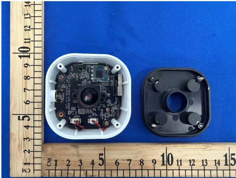
Internal Photos(Models:C690)
