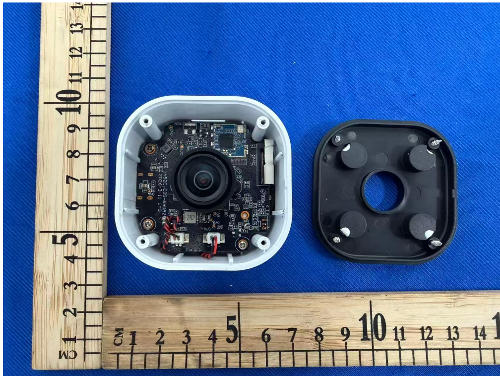
Internal Photos(Models:C692)
