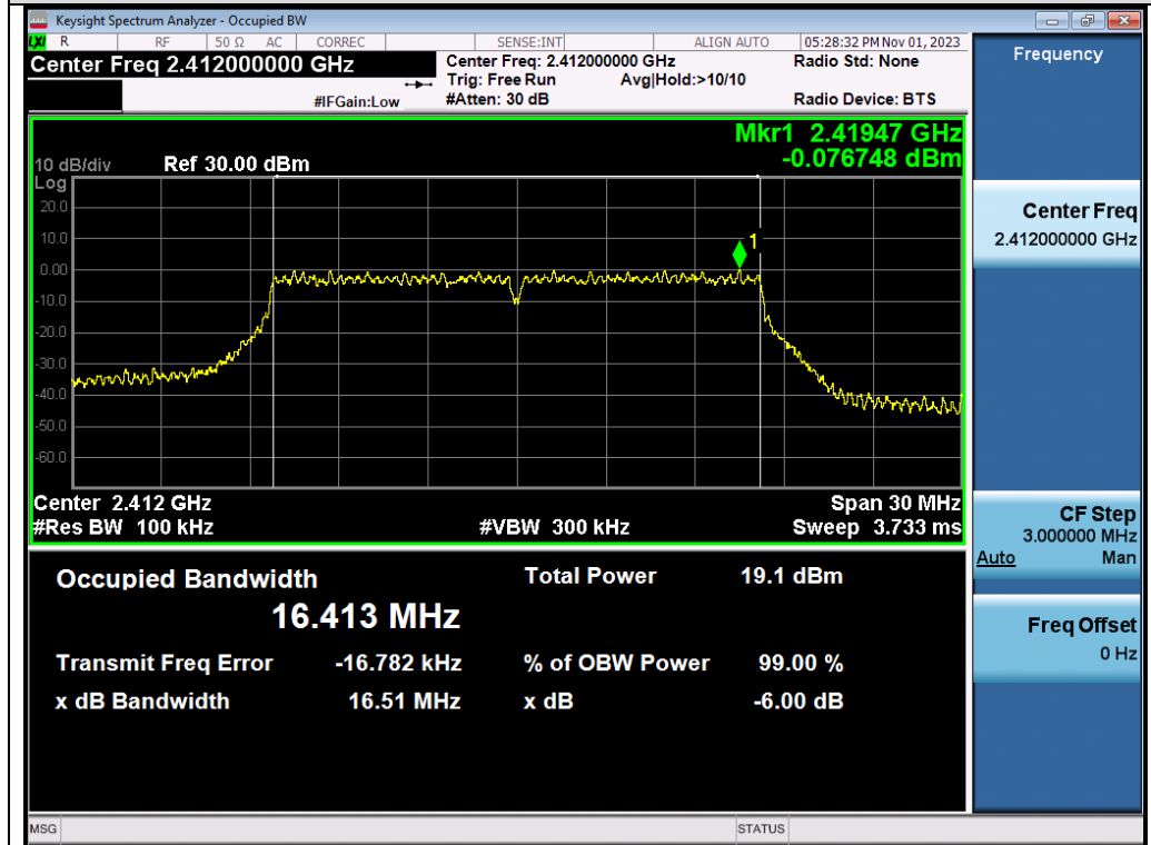
Test_Graph_802.11g_ANT1_2412_54Mbps_DTSBW
