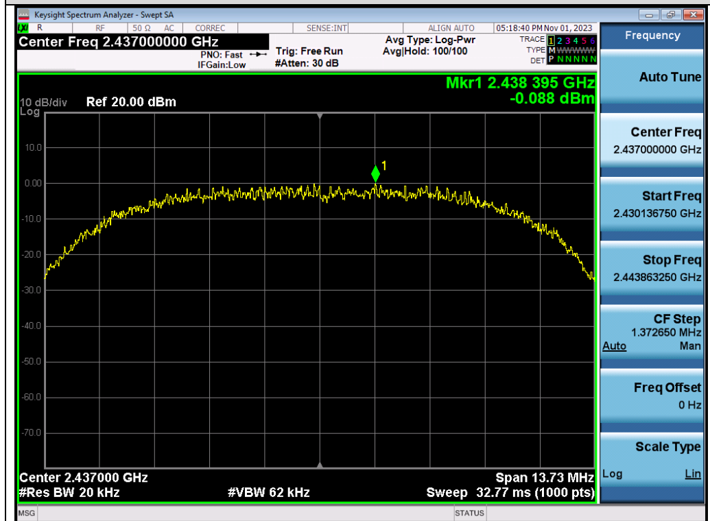
Test_Graph_802.11b_ANT1_2437_11Mbps_PSD
