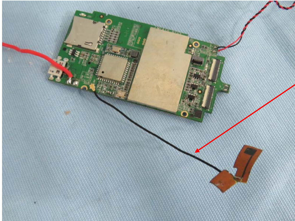
RF Antenna
