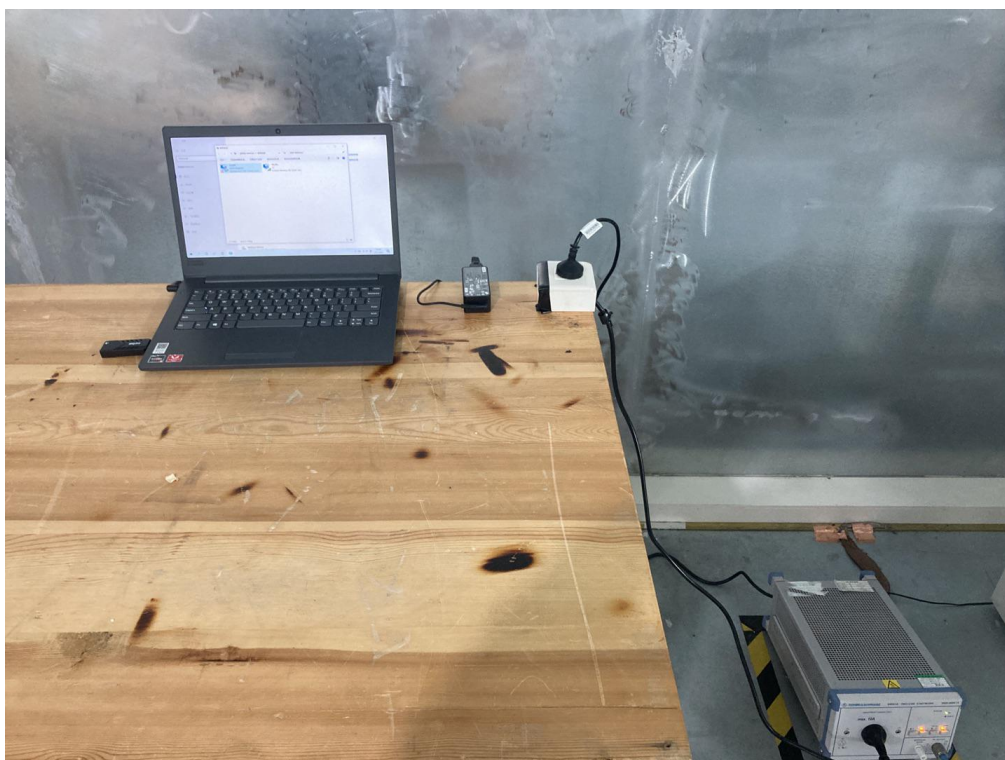
Fig.2(Photo of Power Line Conducted Emission Measurement)
