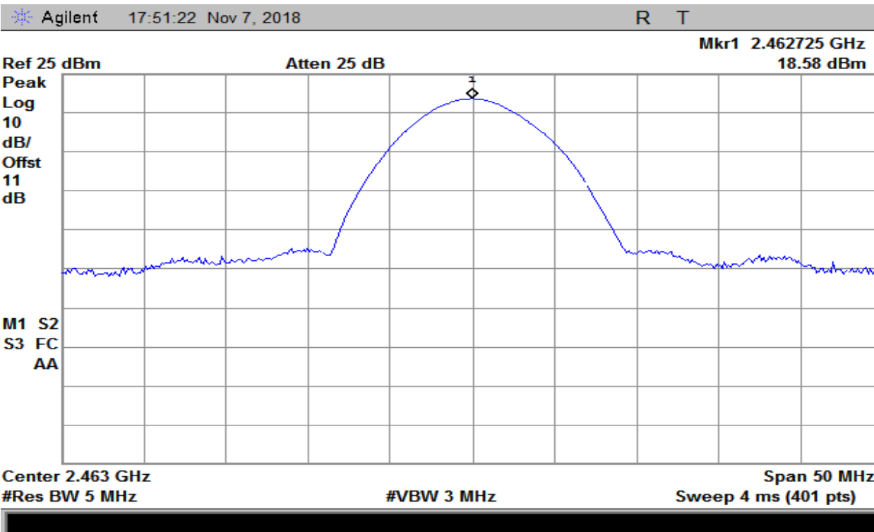
Plot 8 – Output Power – High (Channel # 11)
