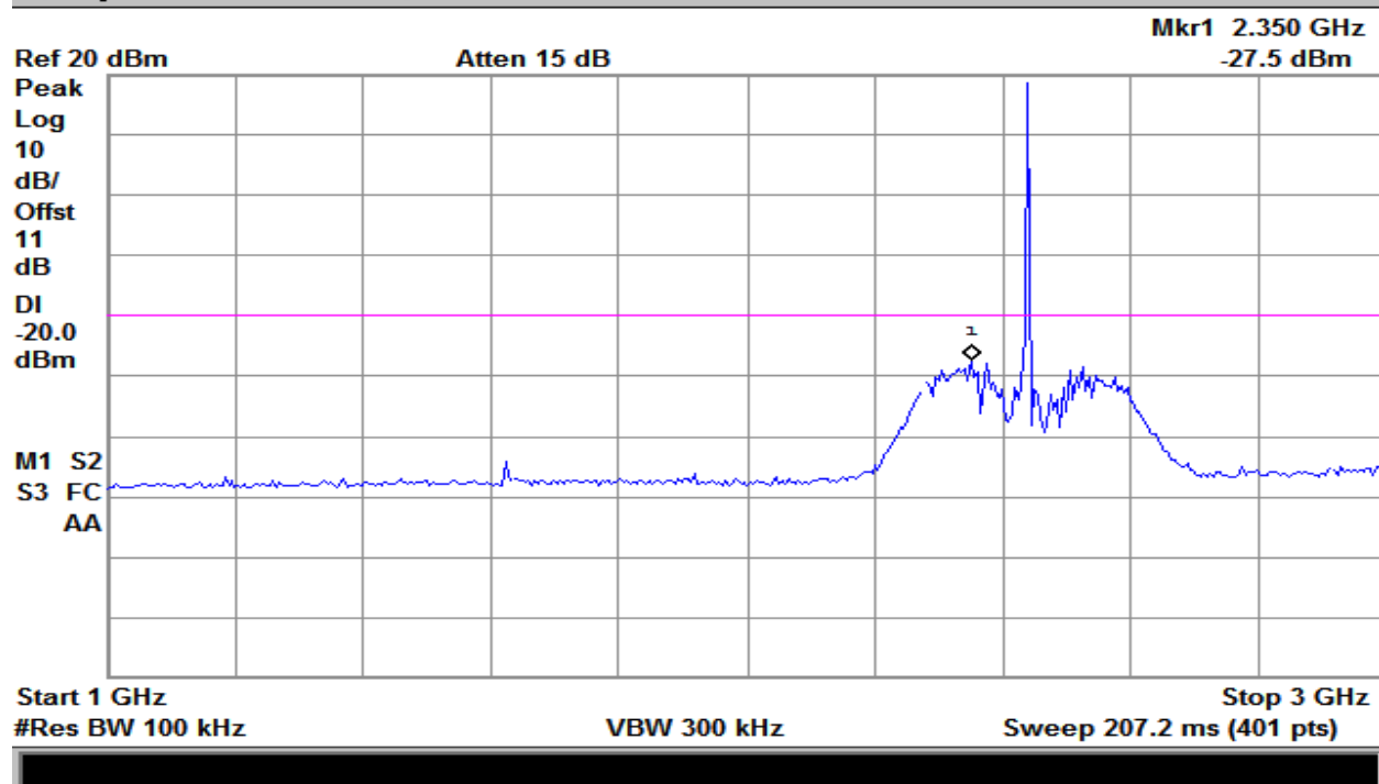
Plot 15 – Mid Band – 1GHz to 3GHz
