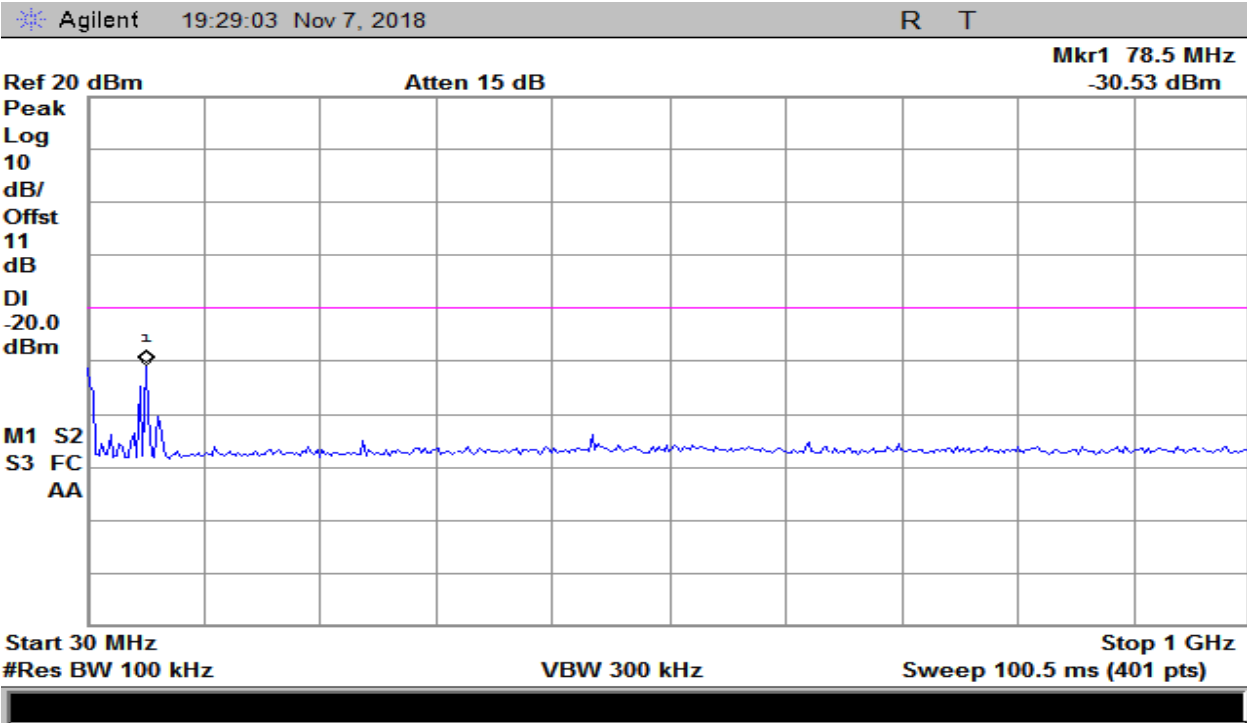
Plot 9 – Low Band – 30MHz to 1GHz
