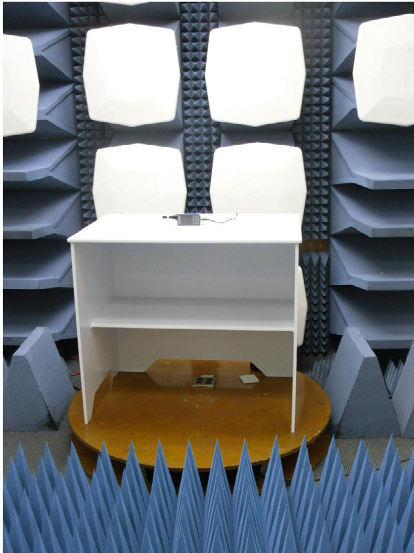
Test Setup Photo # 3
