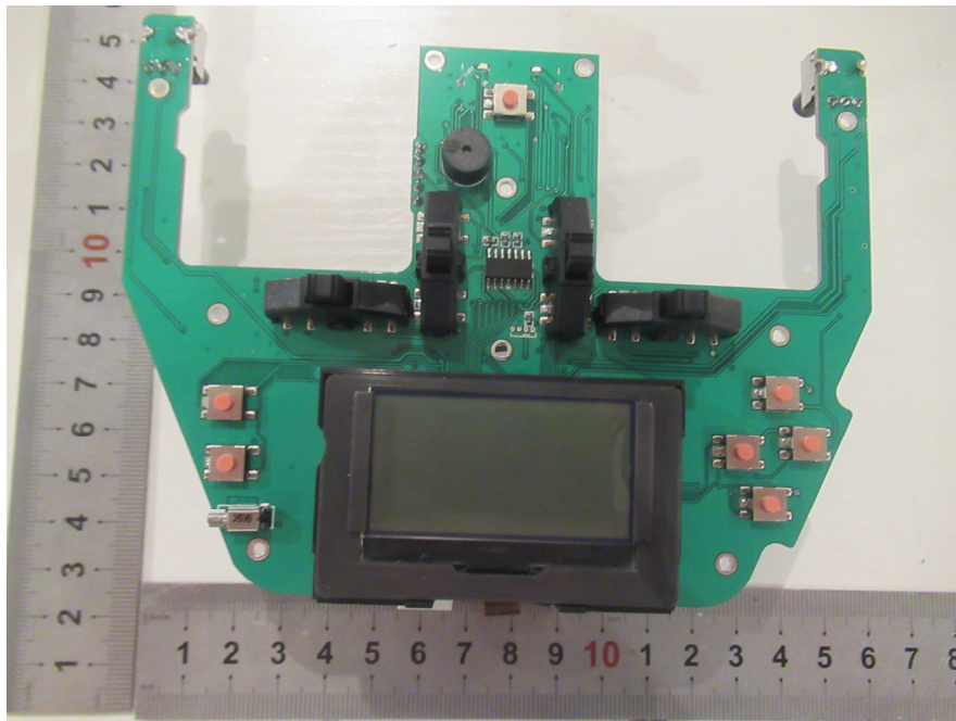
EUT - PCB-2 Screen Removed View
