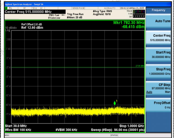
30MHz-1G
