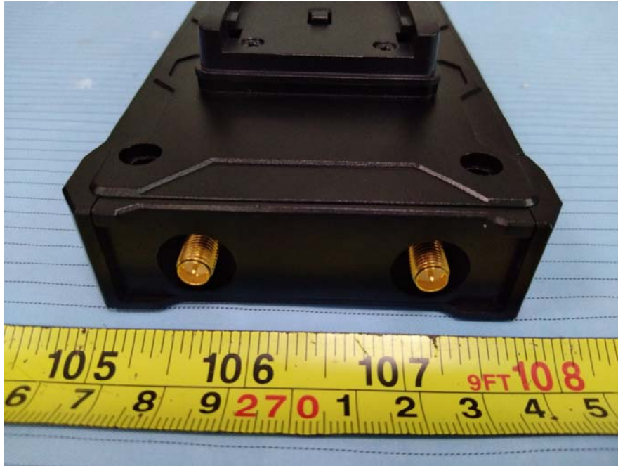
EUT (SH700M) – Top View
