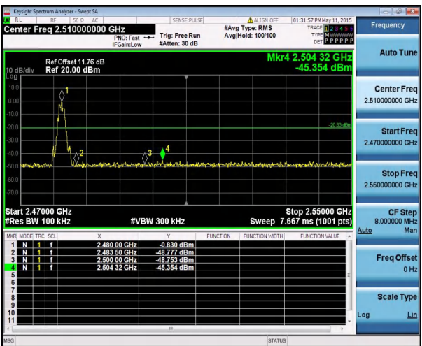
Right bandedge
