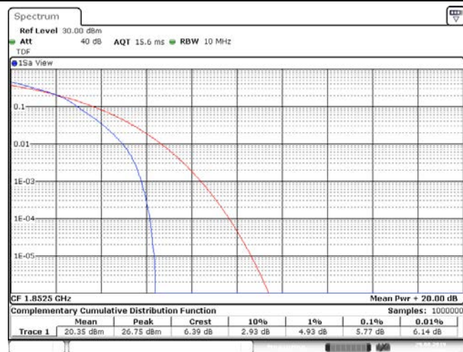
Band25_5MHz_16QAM_26065_25RB#0
