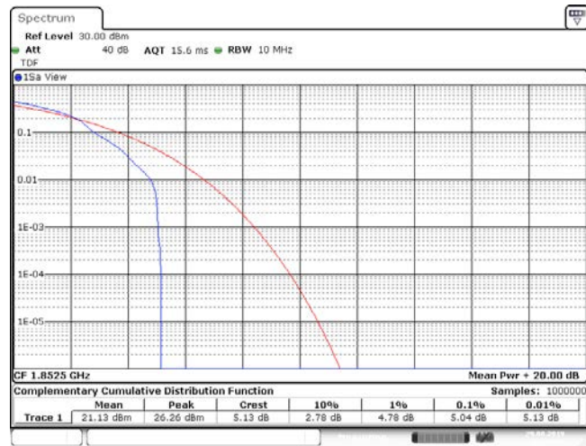
Band25_5MHz_16QAM_26065_1RB#0
