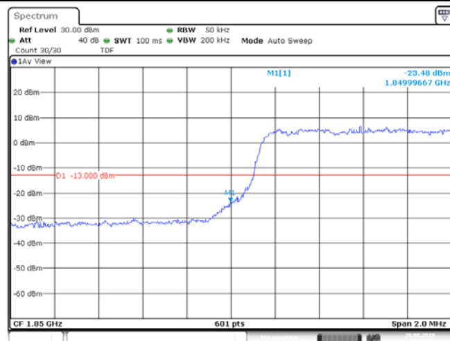
Band25_3MHz_16QAM_26055_15RB#0
