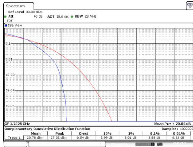
Band4_1.4MHz_16QAM_20175_6RB#0
