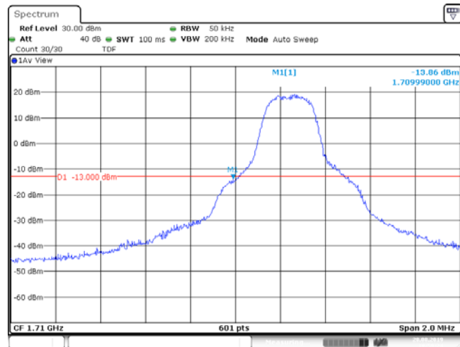
Band4_3MHz_16QAM_19965_1RB#0
