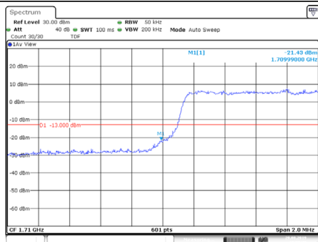
Band4_3MHz_16QAM_19965_15RB#0
