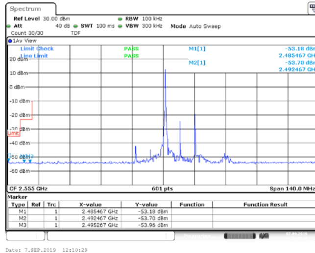
Band41_15MHz_16QAM_40315_1RB#74
