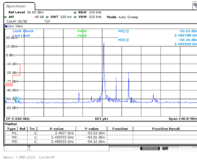
Band41_20MHz_QPSK_40340_1RB#99
