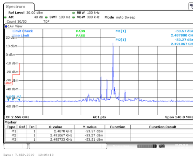
Band41_10MHz_16QAM_40290_50RB#0
