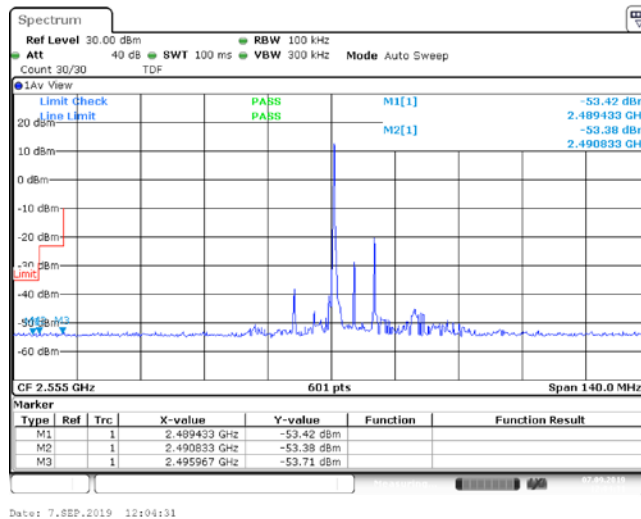
Band41_10MHz_QPSK_40290_1RB#49
