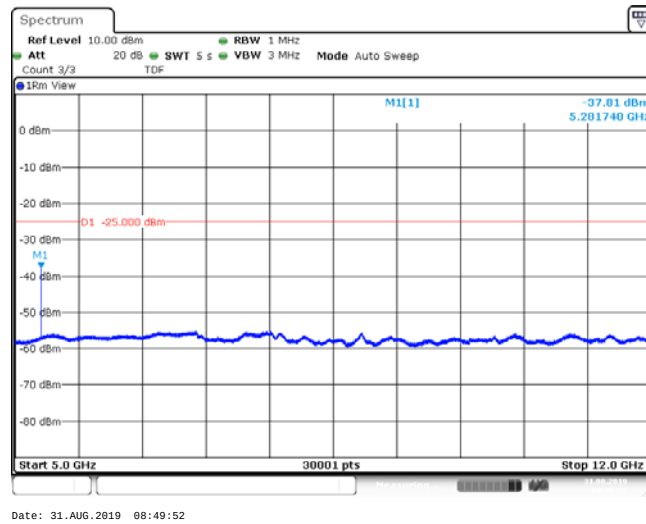
Band41_15MHz_QPSK_41165_1RB#0
