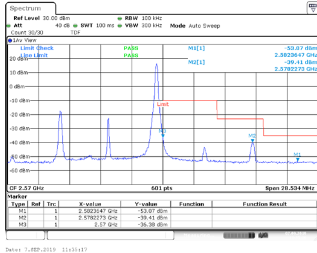
Band7_10MHz_16QAM_21400_50RB#0
