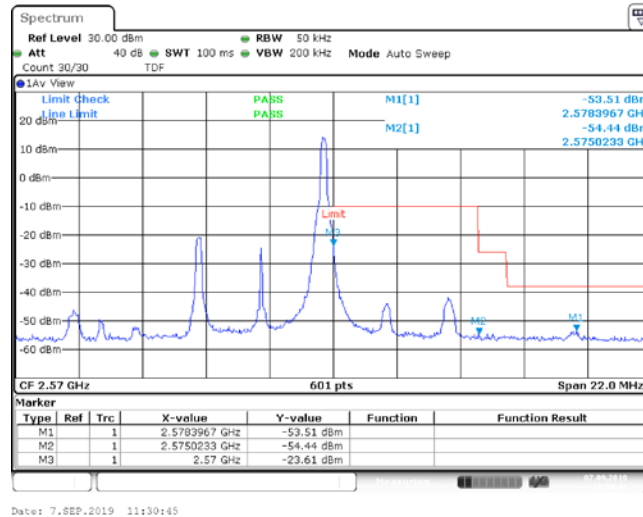
Band7_5MHz_16QAM_21425_25RB#0
