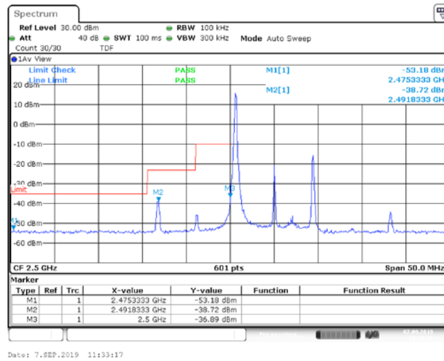
Band7_10MHz_16QAM_20800_50RB#0
