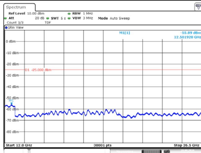
Band7_5MHz_16QAM_21425_1RB#0
