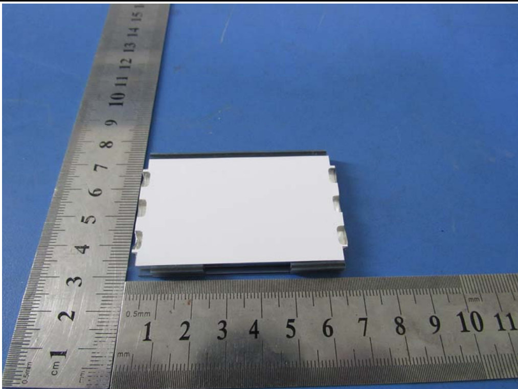
EUT - LCD Rear View
