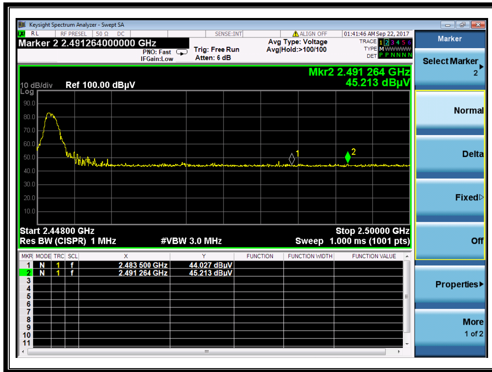
(Plot C1: Channel = 1 PEAK)
