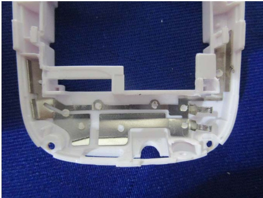
EUT –GSM&FM Antenna View
