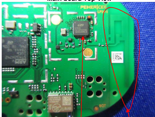
Antenna and RF Chip View
