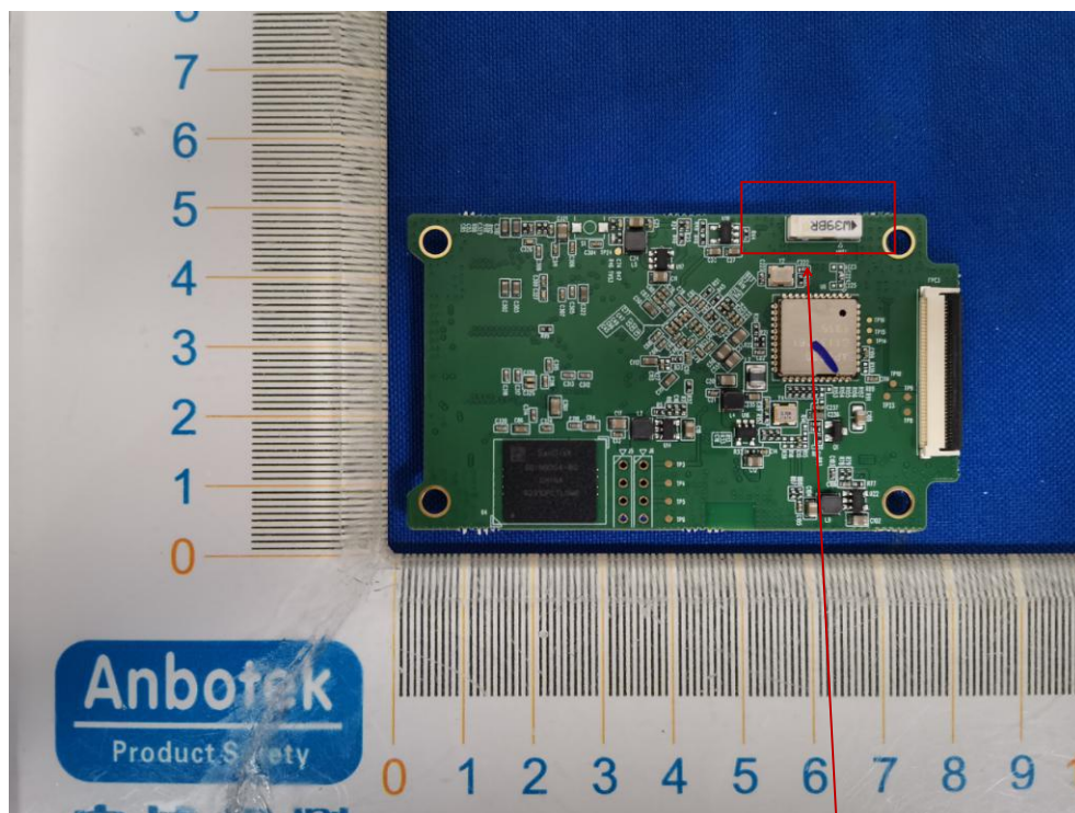
WIFI ANT+BT 2 ANT
