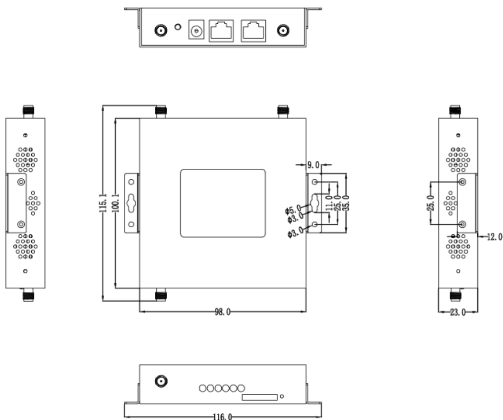
Figure 2-2 S9922M Cellular Wi-Fi Router Figure
