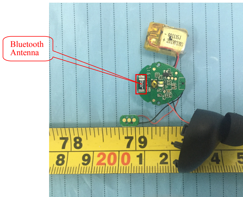
EUT – Main Board Bottom View
