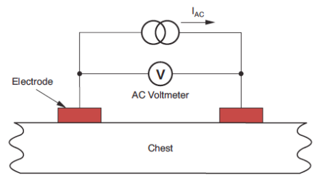
Arrangement of Electrodes for Impedance Pneumography
