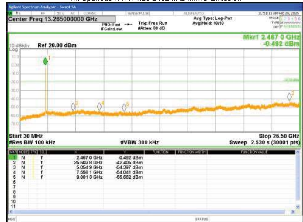
Tx. Spurious NVNT n20 2462MHz MIMO Emission
