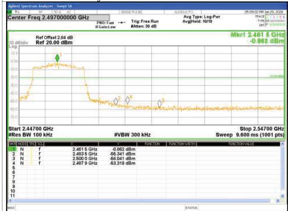
Band Edge NVNT ax20 2462MHz Ant2 Emission
