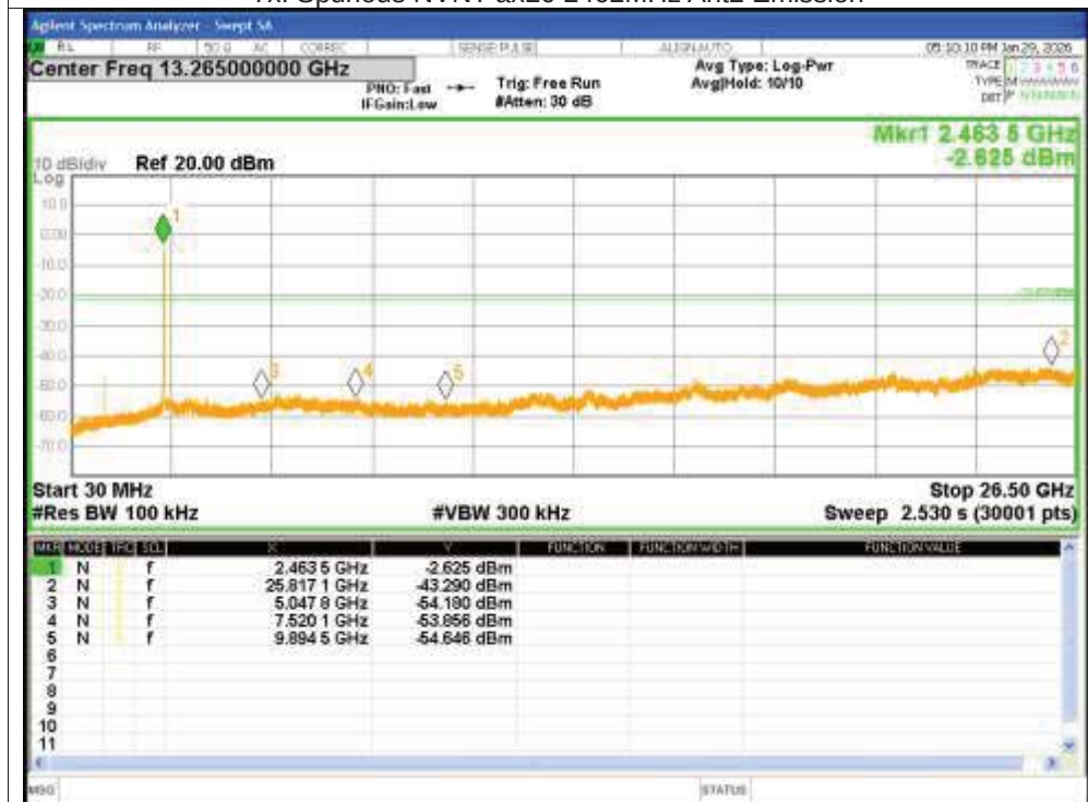
Tx. Spurious NVNT ax20 2462MHz Ant2 Emission
