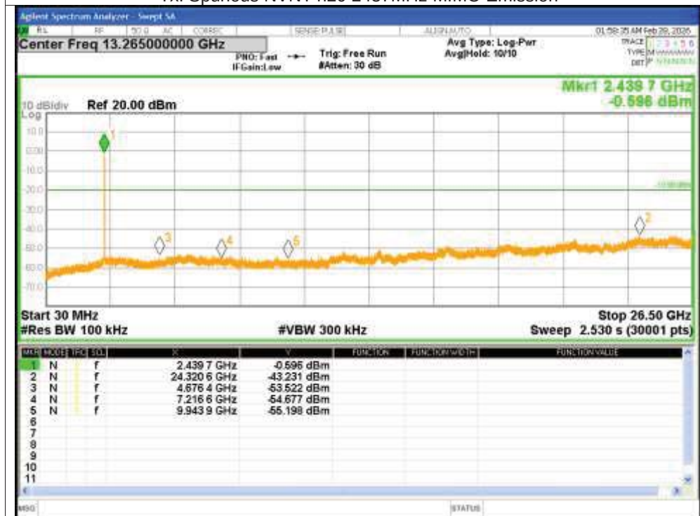
Tx. Spurious NVNT n20 2437MHz MIMO Emission
