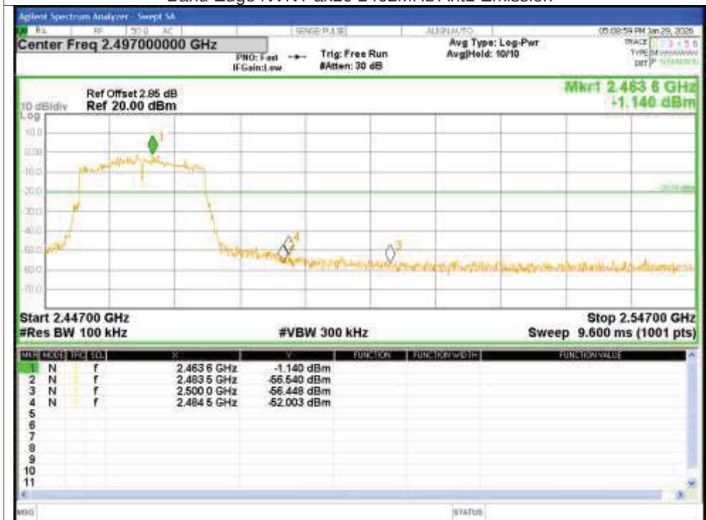
Band Edge NVNT ax20 2462MHz Ant1 Emission
