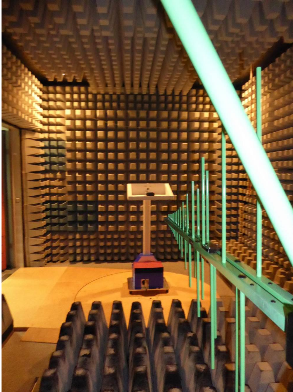
170475_03.JPG: Test setup – radiated test in anechoic chamber
