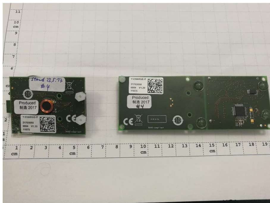
Photograph 4: PCB Bottom side
