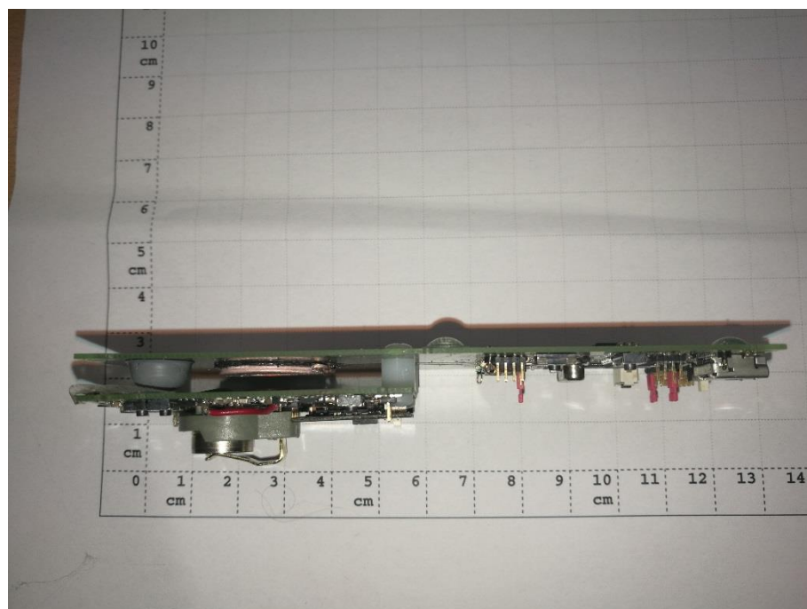
Photograph 3: top side view
