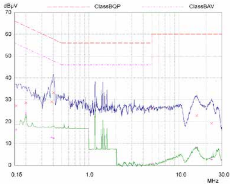
Figure 2 – Line Scan
