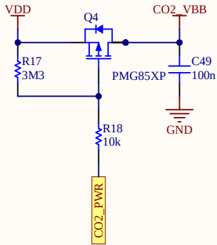
CO2 Sensor Power Supply
