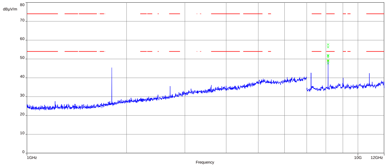
Plot 1: 1 GHz – 12 GHz, horizontal &amp; vertical polarisation (lowest channel)
