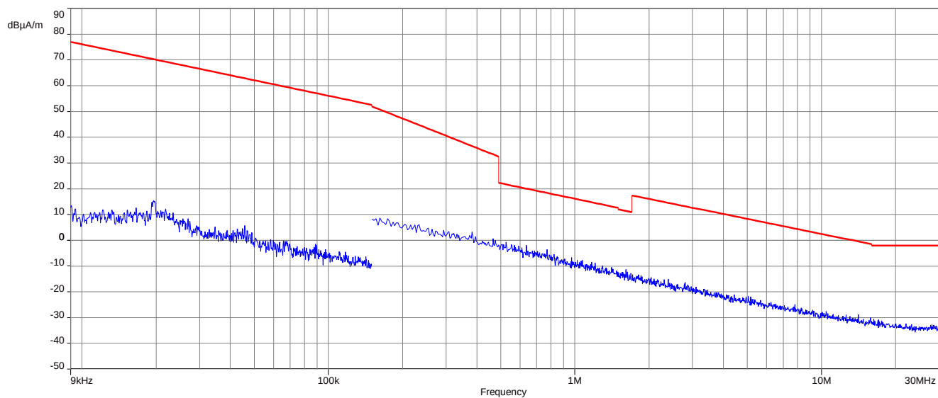
Plot 6: tx-mode high channel, IC
