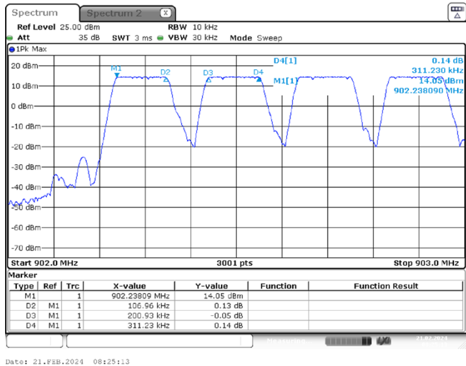
Plot 1: channel separation
