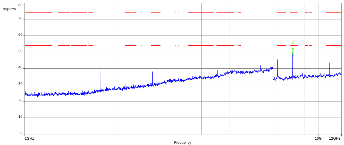
Plot 2: 1 GHz – 12 GHz, horizontal &amp; vertical polarisation (middle channel)
