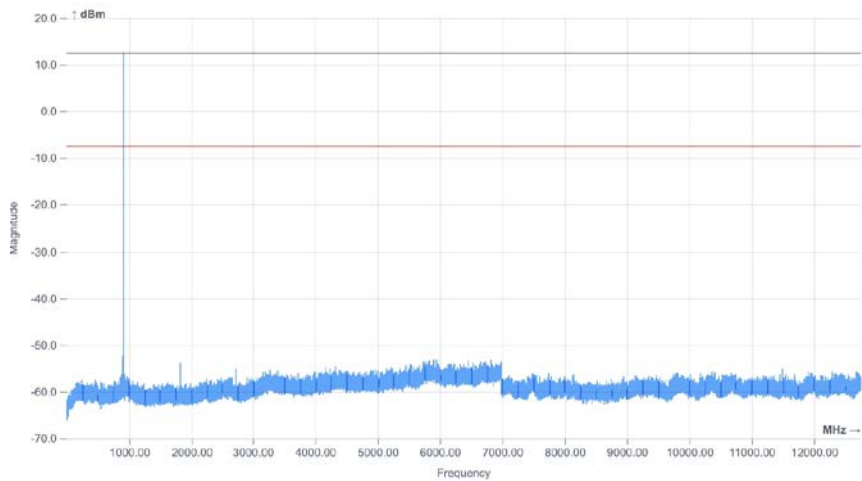
Plot 2: middle channel, 9 kHz – 12.75 GHz
