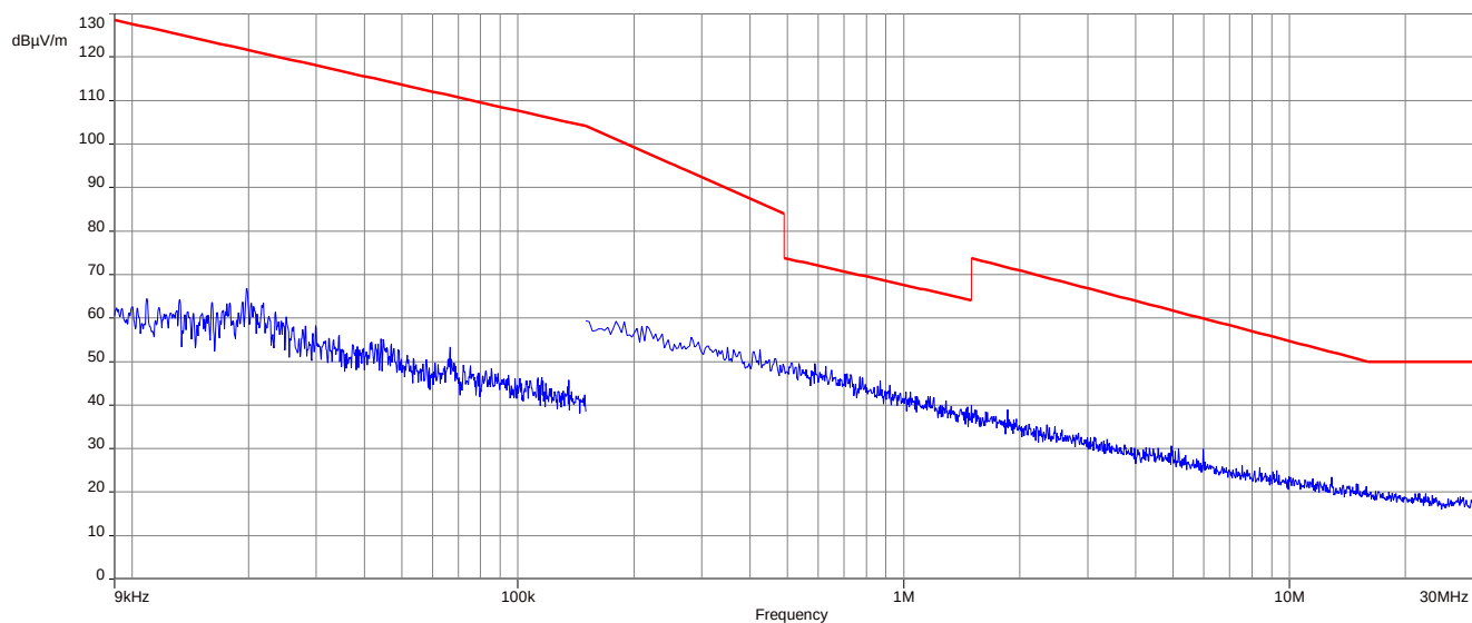
Plot 5: tx-mode high channel, FCC
