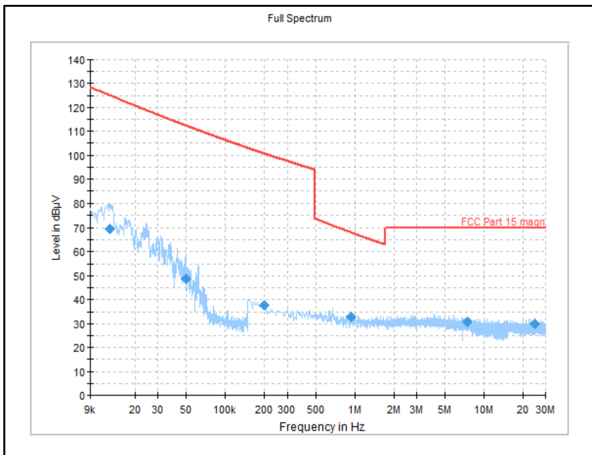
Plot: 9 kHz – 30 MHz: Bluetooth Lowe Energy / Middle Channel
