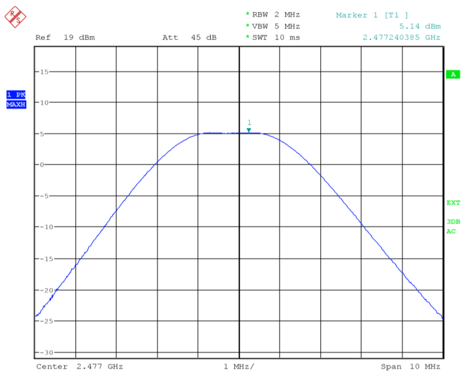
Figure 8.4-6: Output power on high channel – Antenna port 2
