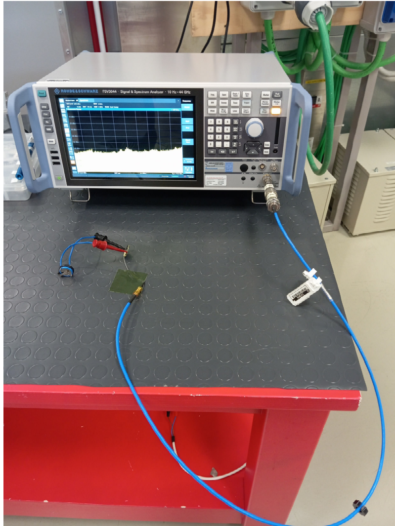
Photo 1 (all conducted tests setups)
