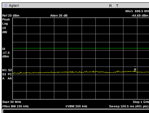
Plot 90. Spurious Conducted Emissions, BT Classic, Type DH5 - 2480 - 30M-1GHz - hopping on
