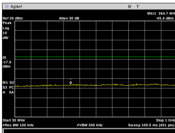
Plot 89. Spurious Conducted Emissions, BT Classic, Type DH5 - 2480 - 30M-1GHz - hopping off
