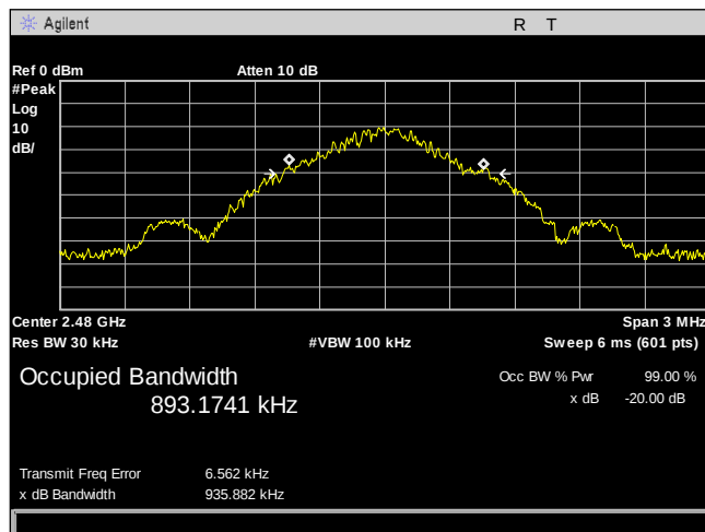
Plot 16. 20 dB Occupied Bandwidth, BT EDR - DH5 - 2480 MHz
