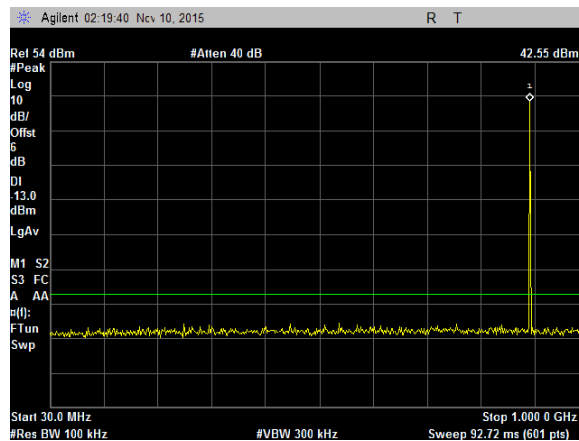
Plot 15. Spurious Emissions at Antenna Terminals, GSM 850, Mid Channel, 30 MHz - 1 GHz
