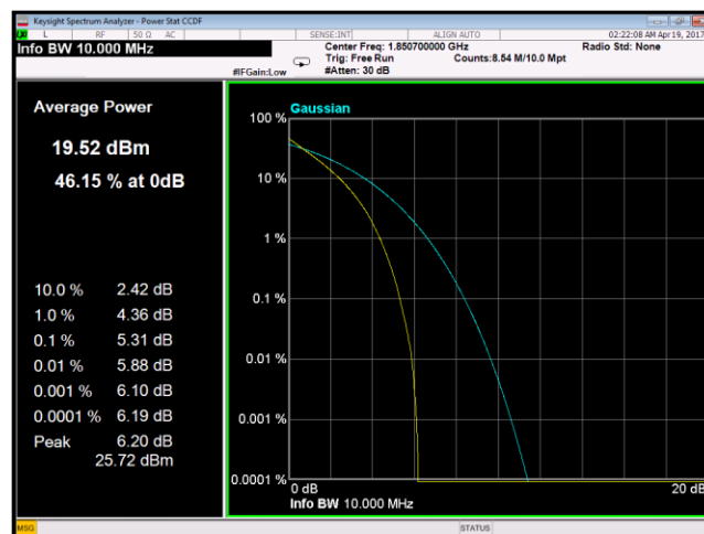
Plot 66. Peak to Average Ratio, Band 2, 1.4MHz, Low Channel
