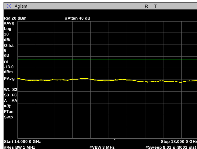
Plot 54. Spurious Emissions at Antenna Terminals, Mid Channel, 1.4MHz, 14 GHz – 18 GHz
