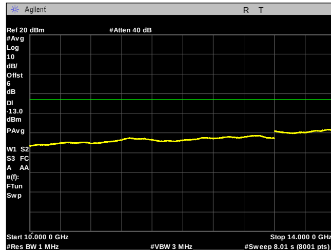
Plot 53. Spurious Emissions at Antenna Terminals, Mid Channel, 1.4MHz, 10 GHz – 14 GHz
