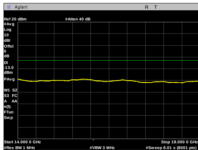
Plot 40. Spurious Emissions at Antenna Terminals, Low Channel, 1.4MHz BW, 14 GHz – 18 GHz
