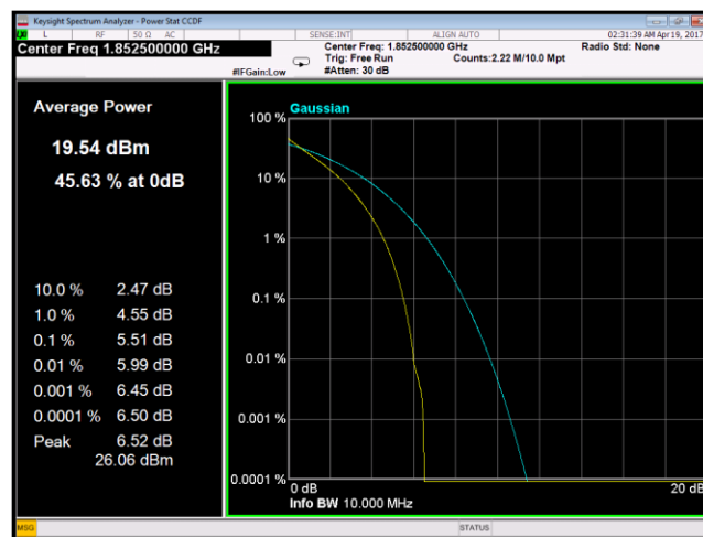
Plot 72. Peak to Average Ratio, Band 2, 5MHz, Low channel
