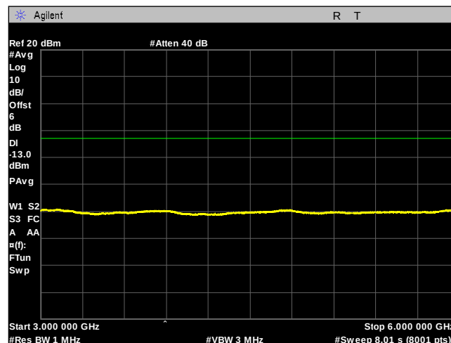
Plot 44. Spurious Emissions at Antenna Terminals, High Channel, 20MHz BW, 3 GHz- 6 GHz
