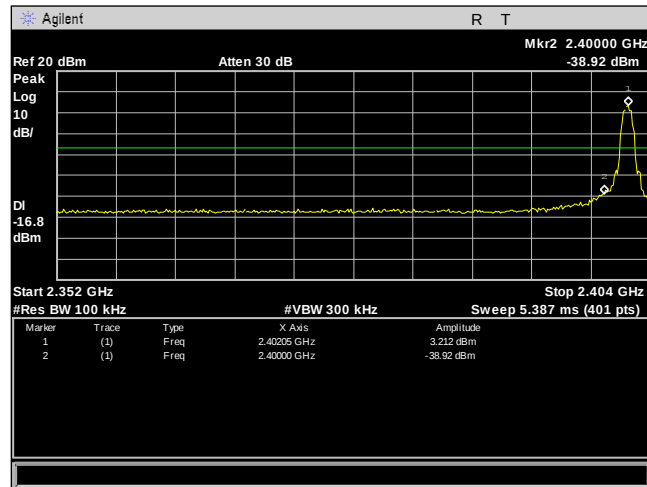
Plot 37. Conducted Band Edge, BT LE - 2402
