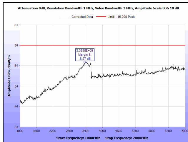
Plot 20. Spurious Radiated Emissions, BT LE - 2480MHz - 1-7GHz - Peak
