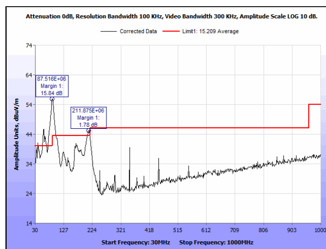
Plot 12. Spurious Radiated Emissions, BT LE - 2402 - 30M-1GHz - QP
