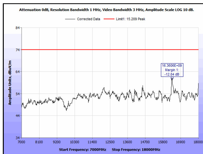
Plot 22. Spurious Radiated Emissions, BT LE - 2402 - 7-18GHz – Peak
