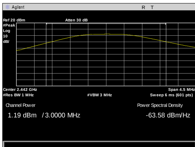
Plot 9. Peak Power Output, BT LE - 2442
