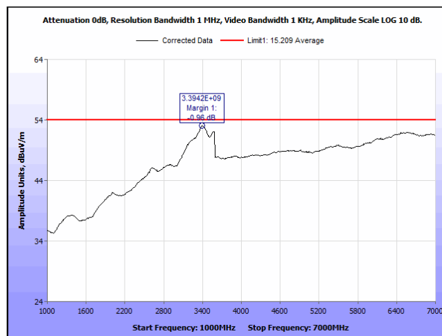
Plot 15. Spurious Radiated Emissions, BT LE - 2402MHz - 1-7GHz - Avg
