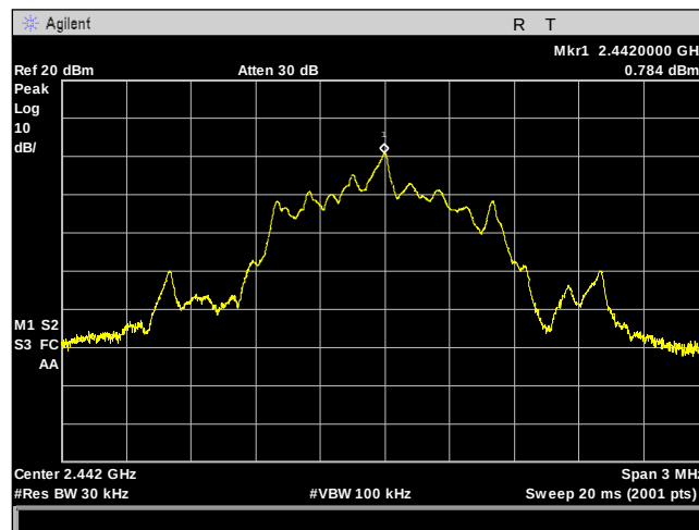
Plot 40. Power Spectral Density, BT LE - 2442
