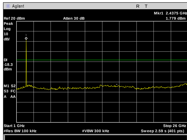
Plot 33. Conducted Spurious Emissions, BT LE - 2442 - 1-26GHz
