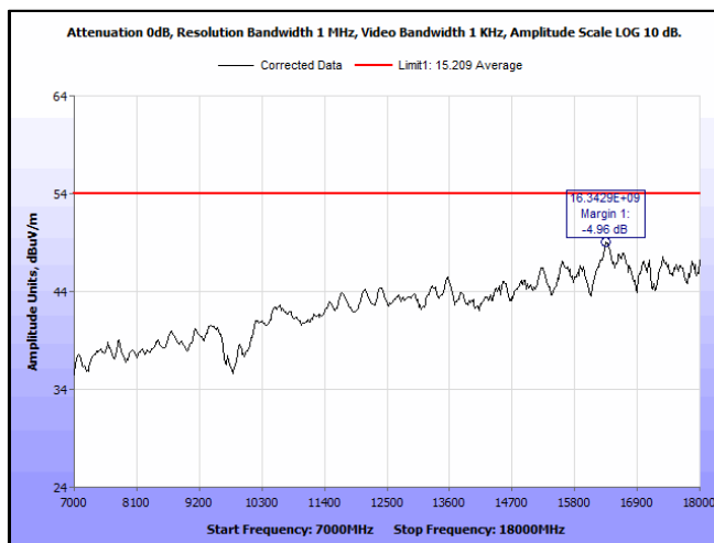
Plot 21. Spurious Radiated Emissions, BT LE - 2402 - 7-18GHz – Avg
