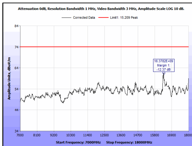
Plot 24. Spurious Radiated Emissions, BT LE - 2442 - 7-18GHz – Peak
