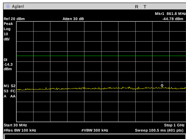
Plot 36. Conducted Spurious Emissions, BT LE - 2480 - 30M-1GHz
