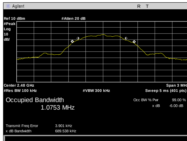
Plot 7. Occupied Bandwidth, LE 2480MHz
