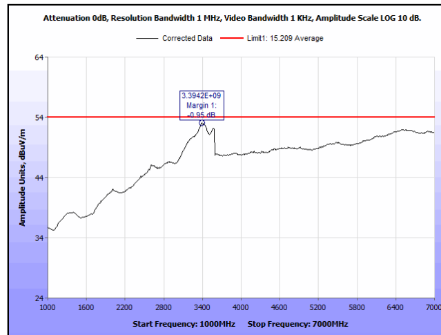
Plot 17. Spurious Radiated Emissions, BT LE - 2442MHz - 1-7GHz - Avg
