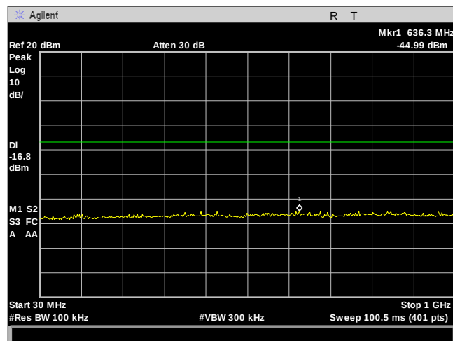
Plot 32. Conducted Spurious Emissions, BT LE - 2402 - 30M-1GHz
