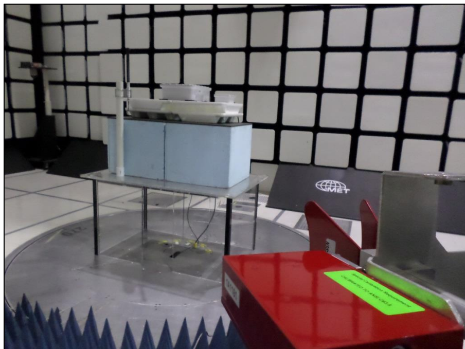
Photograph 10. Radiated Spurious Emissions, 6dBi, 18 - 40 GHz, Test Setup, Antenna
