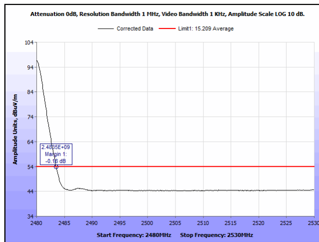
Plot 29. Radiated Restricted Band Edge, BT LE, 2480 MHz, Average
