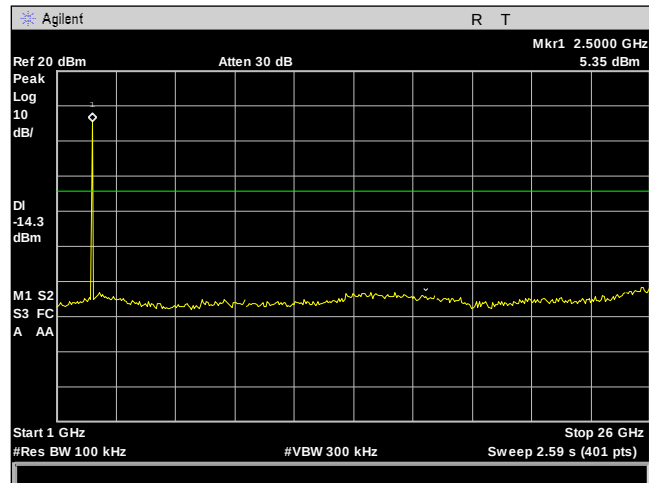
Plot 35. Conducted Spurious Emissions, BT LE - 2480 - 1-26GHz
