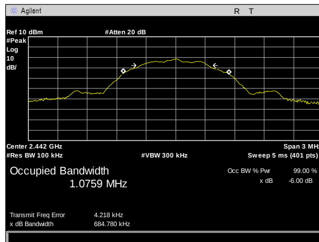
Plot 6. Occupied Bandwidth, LE 2442MHz
