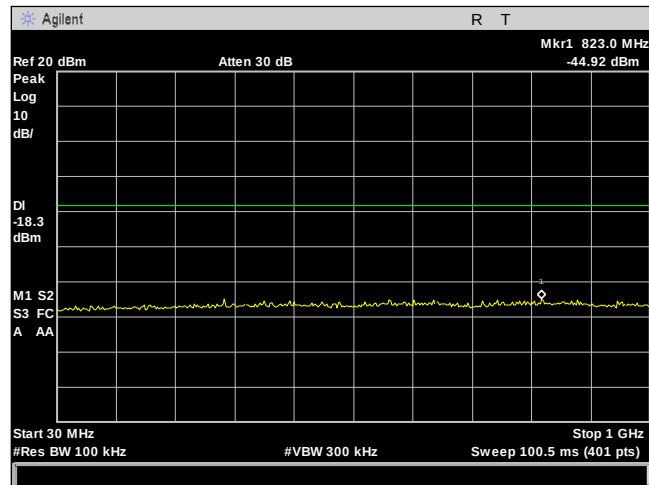
Plot 34. Conducted Spurious Emissions, BT LE - 2442 - 30M-1GHz
