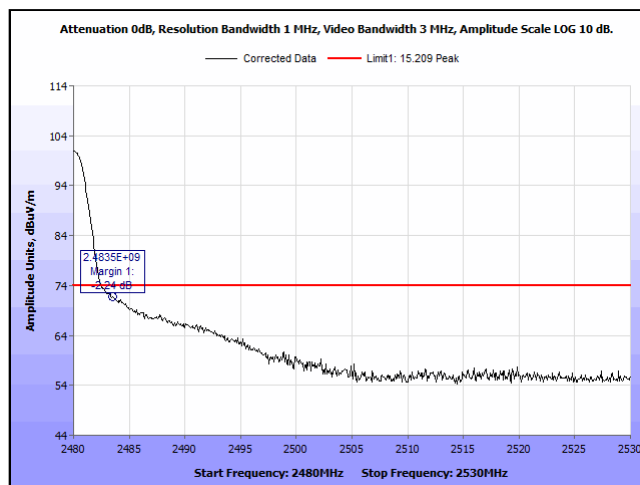
Plot 30. Radiated Restricted Band Edge, BT LE, 2480 MHz, Peak
