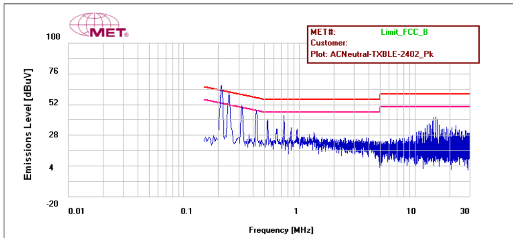
Plot 4. Conducted Emissions, 15.207(a), TX BLE, Neutral Line
