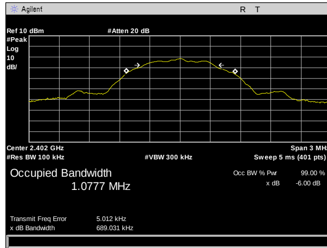
Plot 5. Occupied Bandwidth, LE 2402MHz
