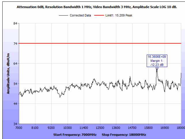
Plot 26. Spurious Radiated Emissions, BT LE - 2480 - 7-18GHz - Peak
