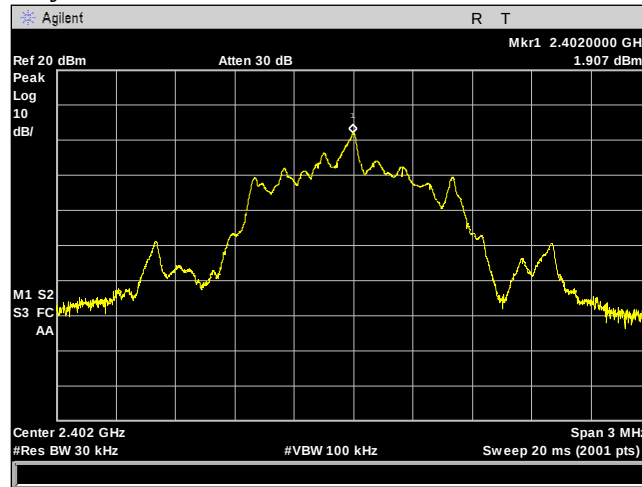
Plot 39. Power Spectral Density, BT LE - 2402
