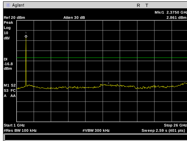
Plot 31. Conducted Spurious Emissions, BT LE - 2402 - 1-26GHz
