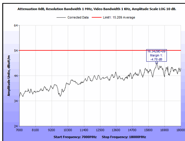
Plot 25. Spurious Radiated Emissions, BT LE - 2480 - 7-18GHz – Avg
