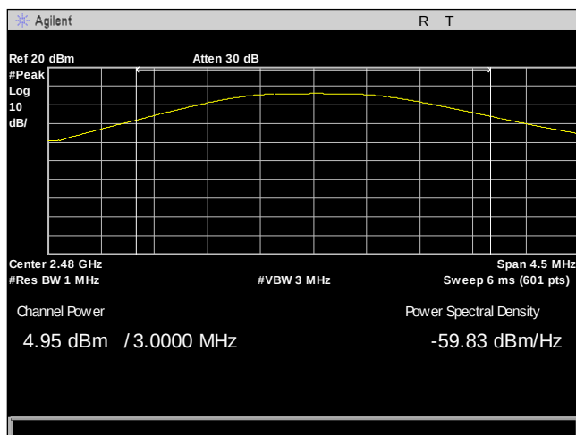
Plot 10. Peak Power Output, BT LE - 2480
