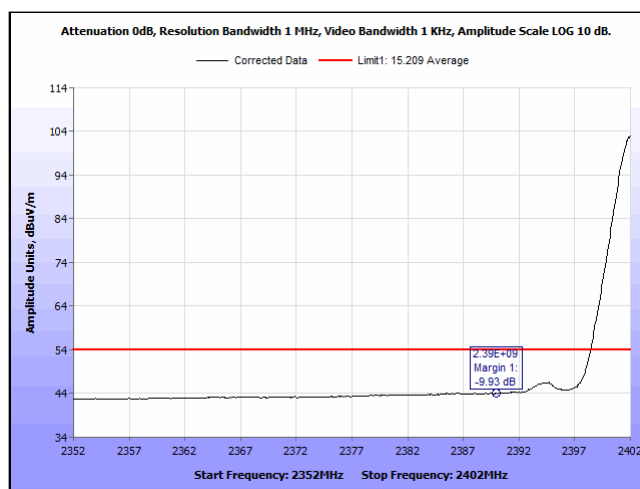
Plot 27. Radiated Restricted Band Edge, 2402 MHz, BT LE, Average
