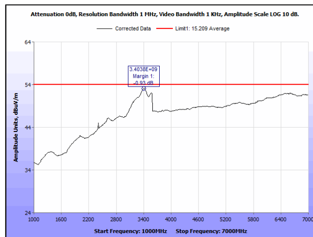
Plot 19. Spurious Radiated Emissions, BT LE - 2480MHz - 1-7GHz - Avg
