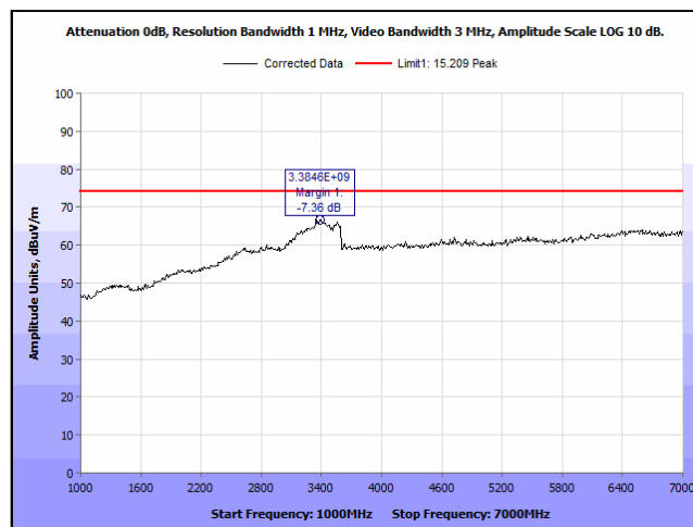
Plot 16. Spurious Radiated Emissions, BT LE - 2402MHz - 1-7GHz - Peak
