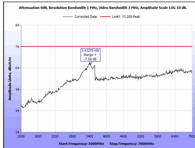
Plot 18. Spurious Radiated Emissions, BT LE - 2442MHz - 1-7GHz - Peak
