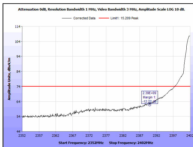
Plot 28. Radiated Restricted Band Edge, BT LE, 2402 MHz, Peak
