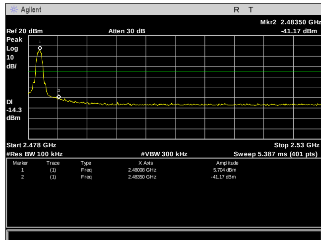
Plot 38. Conducted Band Edge, BT LE - 2480
