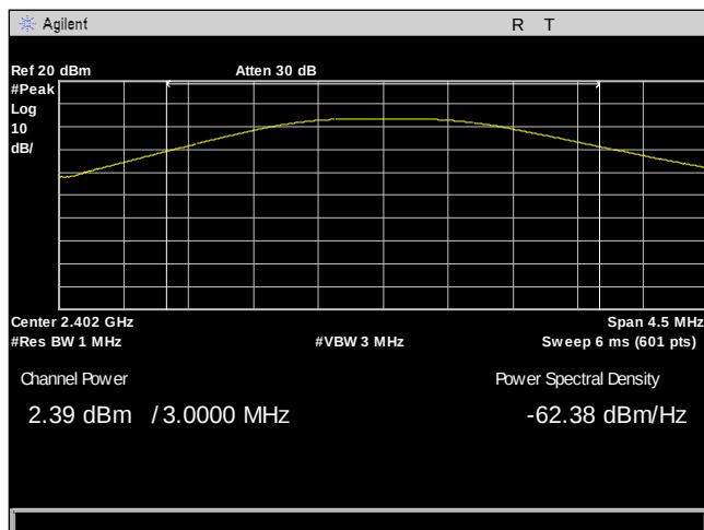
Plot 8. Peak Power Output, BT LE - 2402
