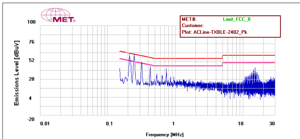
Plot 2. Conducted Emissions, 15.207(a), TX BLE, Phase Line
