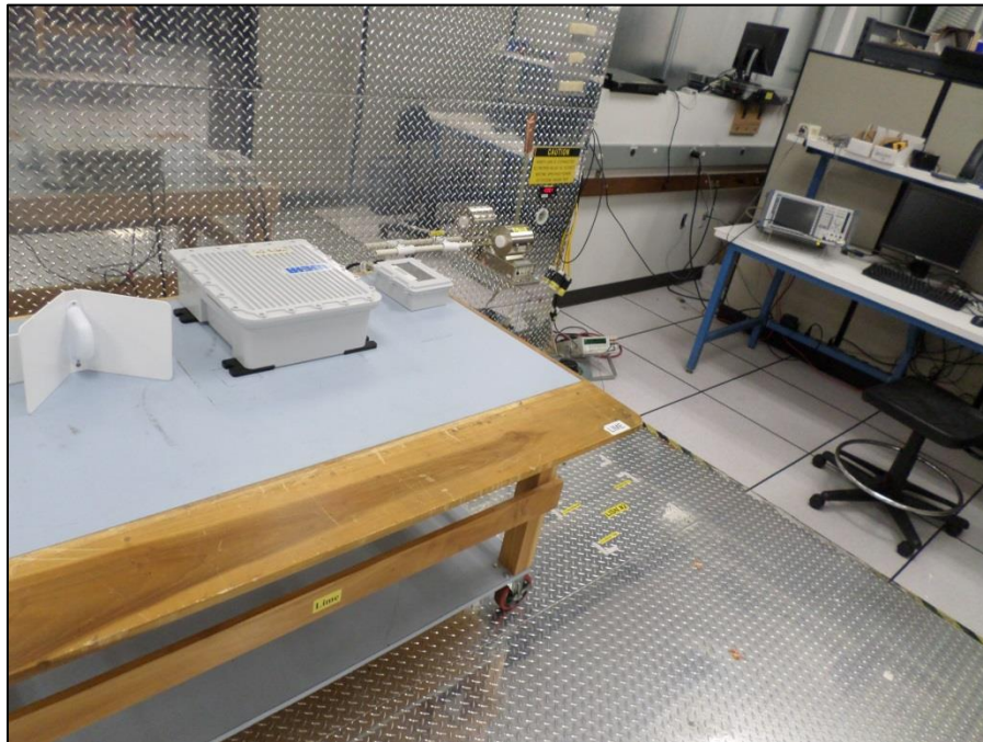
Photograph 1. Conducted Emissions, 15.207(a), Station Setup
