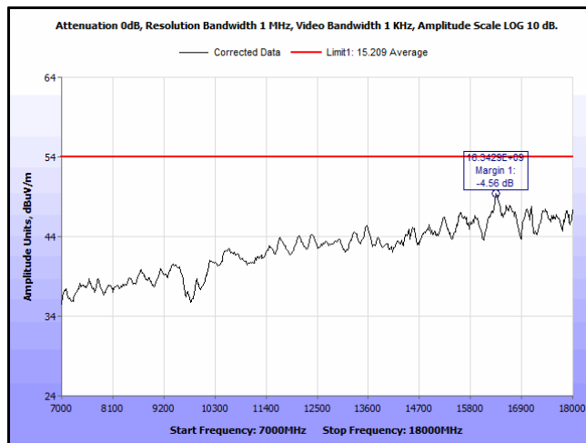
Plot 23. Spurious Radiated Emissions, BT LE - 2442 - 7-18GHz – Avg
