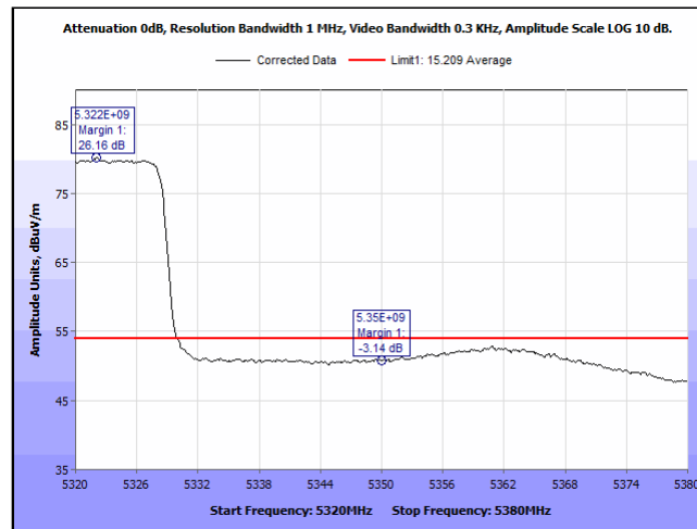
Plot 318. Radiated Band Edge, 5280 MHz, AC mode, 80 MHz, Average, MIMO
