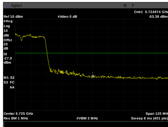
Plot 372. Frequency Stability, 5725 MHz, Band Edge, 40 MHz, Channel Average 80.C
