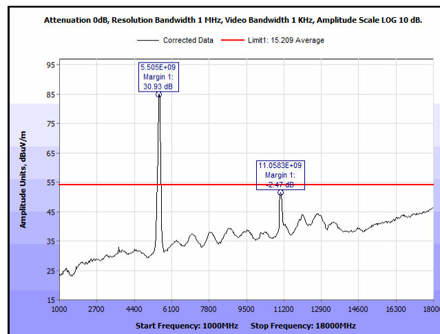
Plot 289. Undesirable Emissions, 1 – 18 GHz, 5530 MHz, AC mode, 80 MHz, Average, MIMO
