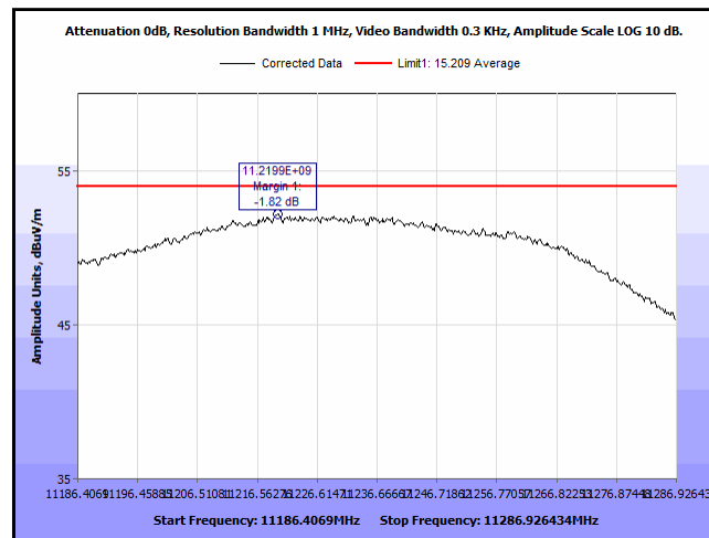
Plot 296. Undesirable Emissions, 1 – 18 GHz, 5610 MHz, 11.2 GHz, AC mode, 80 MHz, Average, MIMO
