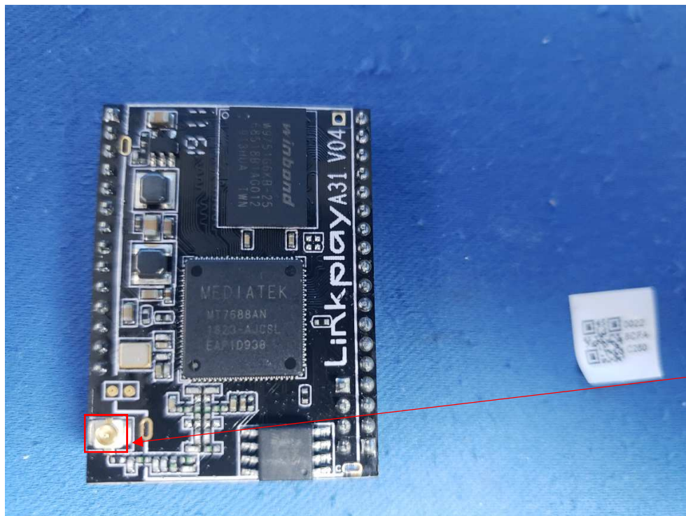
WIFI ANT Port
