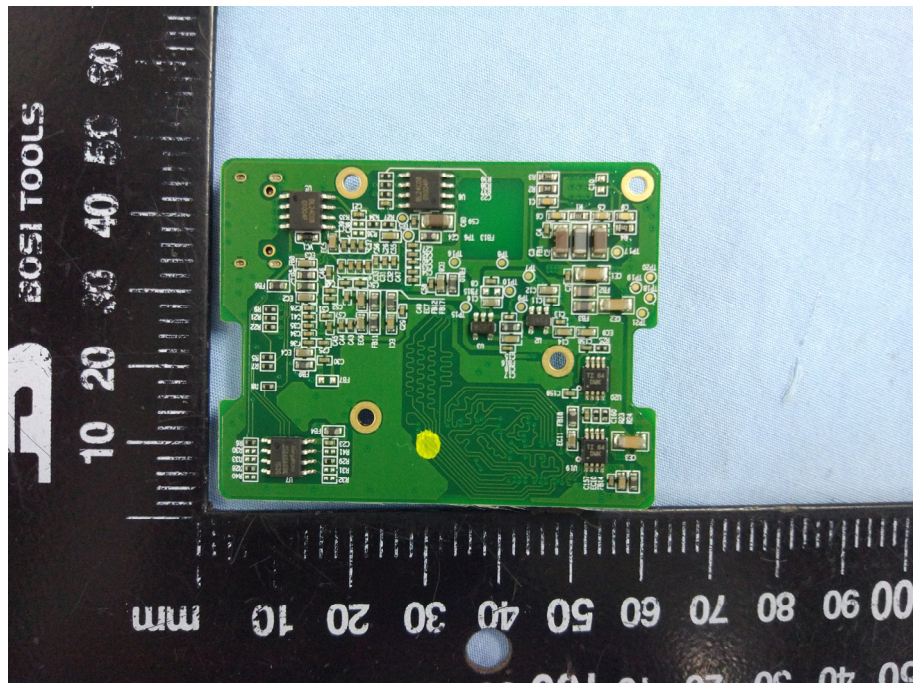
Solder Board-Component View 2(ROBOT-HDMI2RGB)
