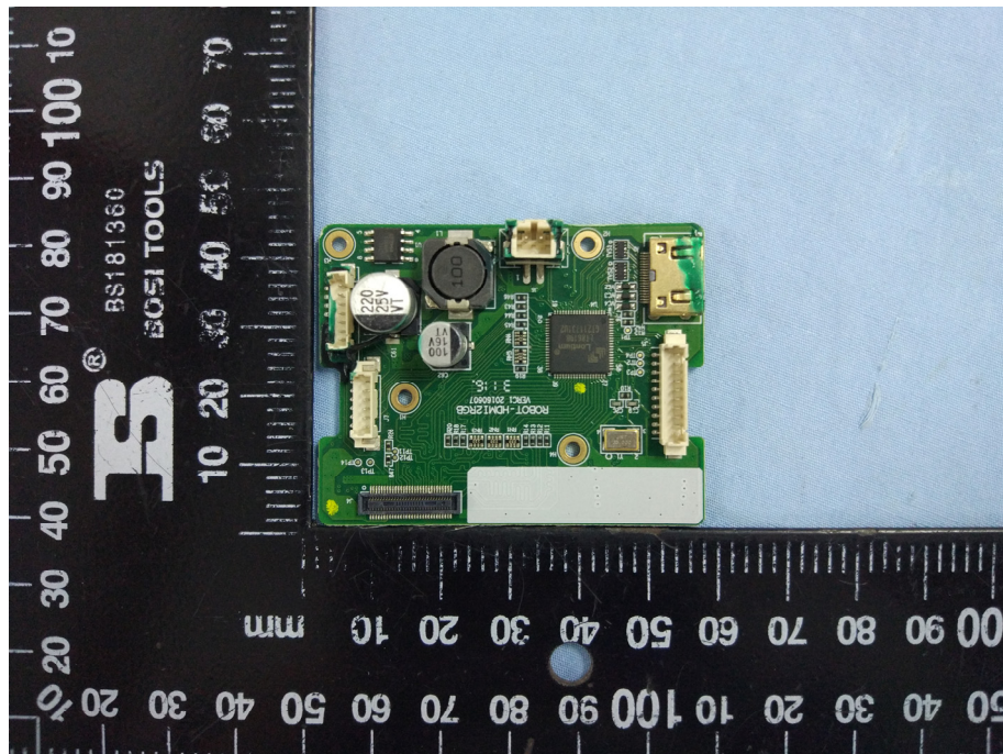
Solder Board-Component View 1(ROBOT-HDMI2RGB)
