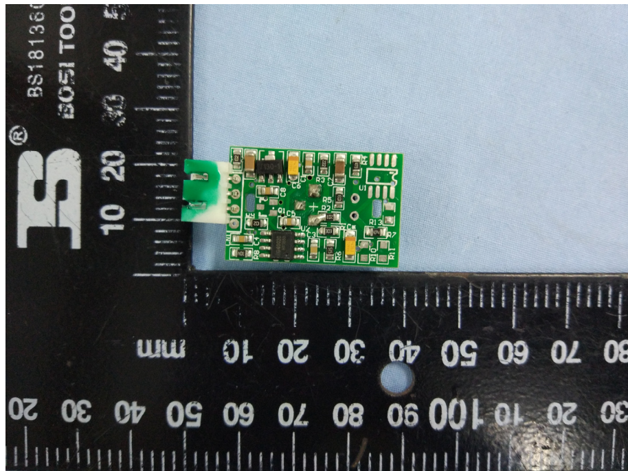
Solder Board-Component View 5(PIR)
